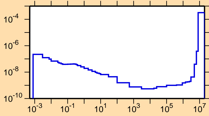
\sigma vs. E for ^{261}\text{No}(n,\alpha)
