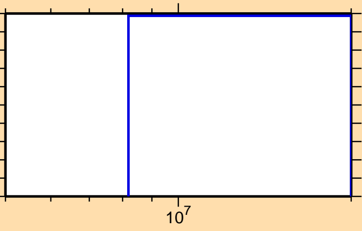
\sigma vs. E for ^{261}\text{No}(n,3n)
