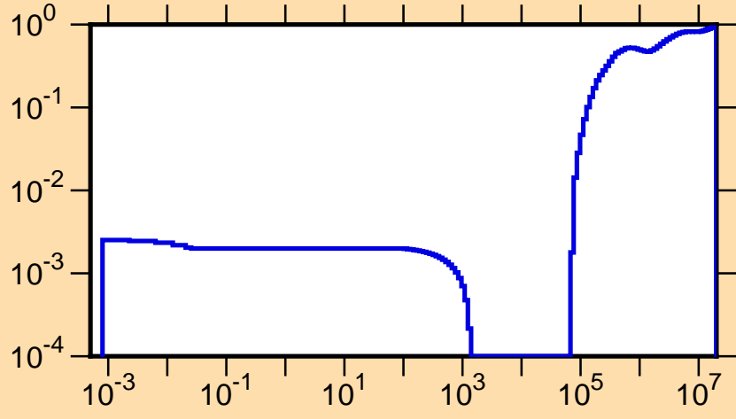
\mu vs. E for ^{263}\text{No}(\text{mt251})
