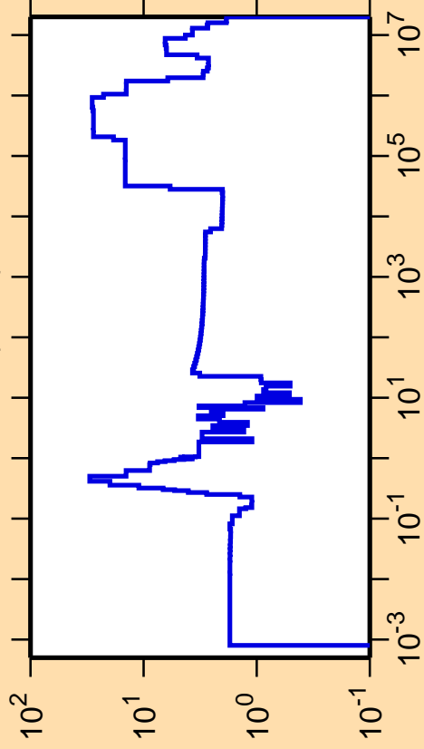
\Delta\sigma/\sigma vs. E for ^{263}\text{No}(n,\text{el.})
