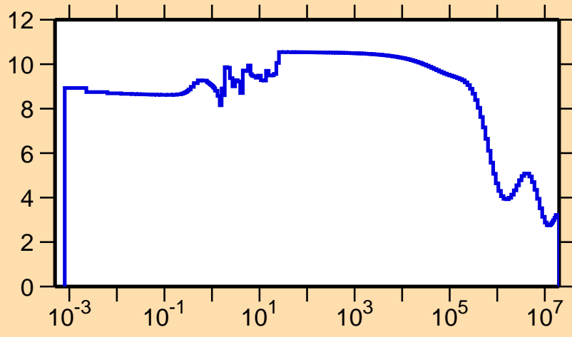
\sigma vs. E for ^{263}\text{No}(n,\text{el.})
