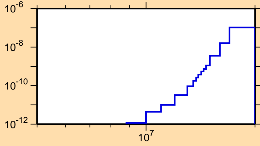
\sigma vs. E for ^{263}\text{No}(n,2n\alpha)
