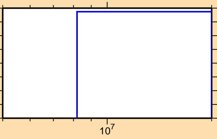
\sigma vs. E for ^{263}\text{No}(n,2np)
