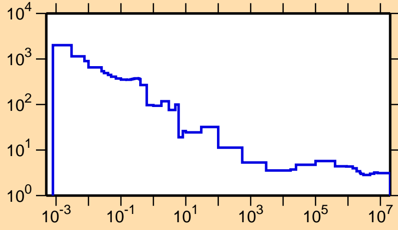
\sigma vs. E for ^{263}\text{No}(n,\text{nonel.})
