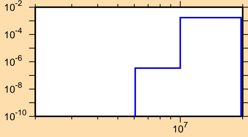
\sigma vs. E for ^{228}\text{Np}(n,d)
