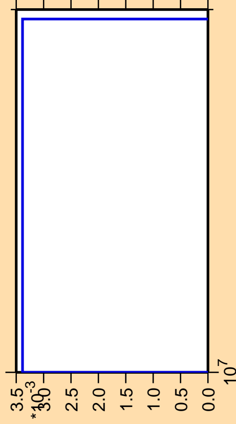
\Delta\sigma/\sigma vs. E for ^{228}\text{Np} (mt 11)
