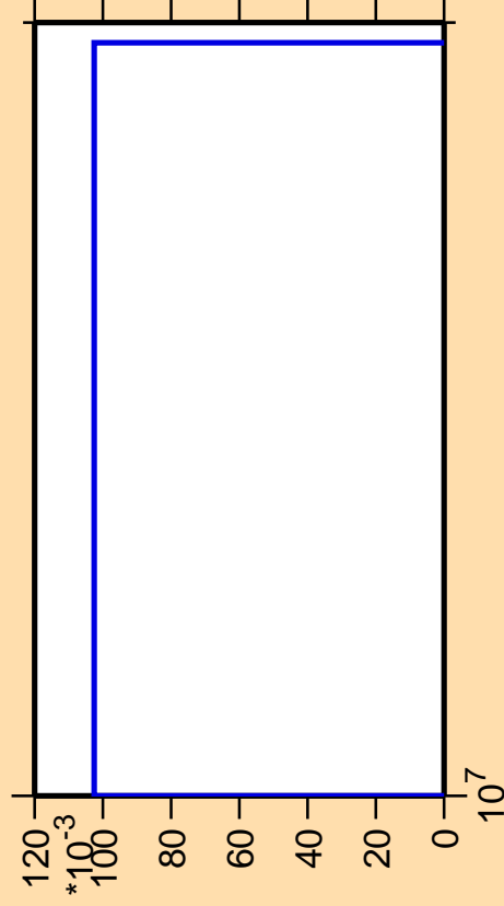
\Delta\sigma/\sigma vs. E for ^{228}\text{Np}(n,pd)
