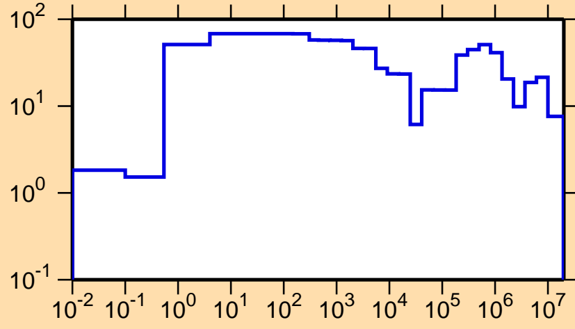
\Delta\sigma/\sigma vs. E for ^{228}\text{Np}(n,el.)
