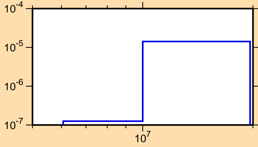
\sigma vs. E for ^{228}\text{Np}(n,2n\alpha)
