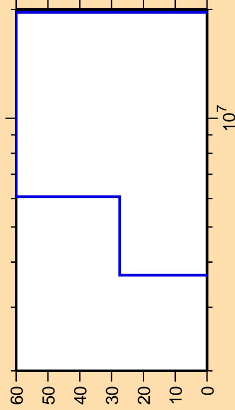
\Delta\sigma/\sigma vs. E for ^{228}\text{Np}(n,d)
