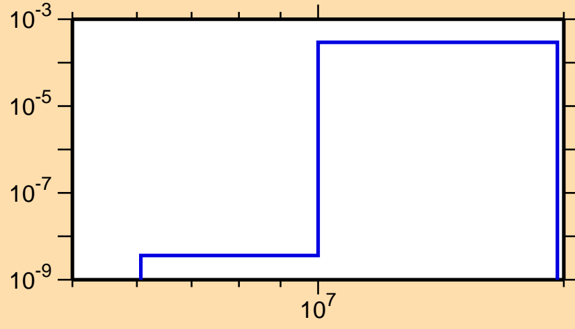
\sigma vs. E for ^{228}\text{Np}(n,t)
