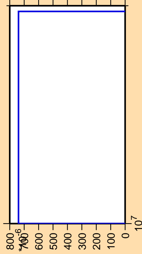
\Delta\sigma/\sigma vs. E for ^{228}\text{Np} (mt 42)
