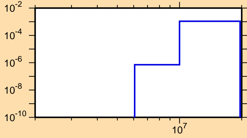
\sigma vs. E for ^{228}\text{Np}(n,np)
