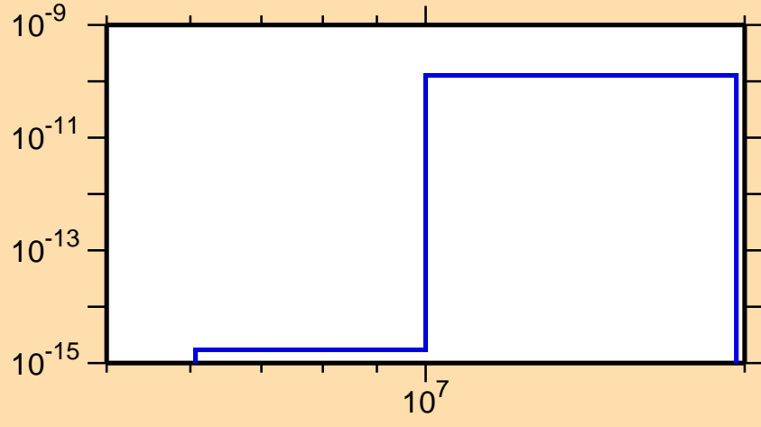
\sigma vs. E for ^{228}\text{Np}(\text{mt117})
