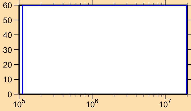
\Delta\sigma/\sigma vs. E for ^{228}\text{Np}(n,n_1)
