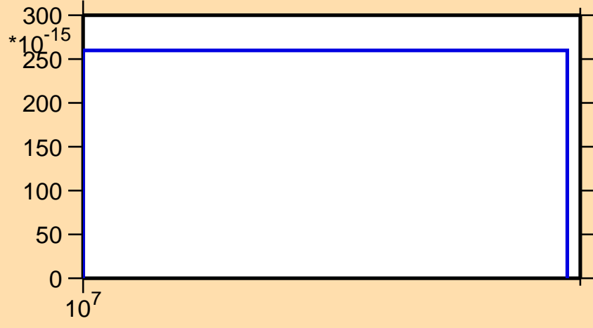
\sigma vs. E for ^{228}\text{Np} (mt 34)
