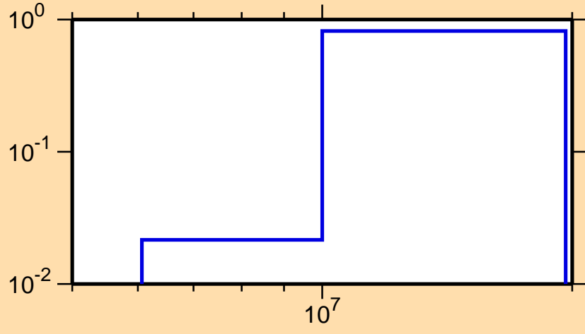
\sigma vs. E for ^{228}\text{Np}(n,2n)
