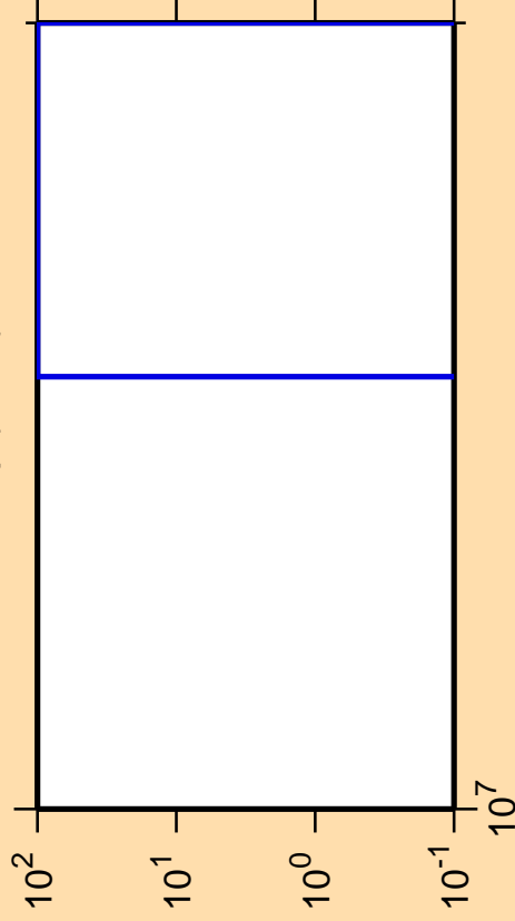
\Delta\sigma/\sigma vs. E for ^{229}\text{Np}(n,3n)
