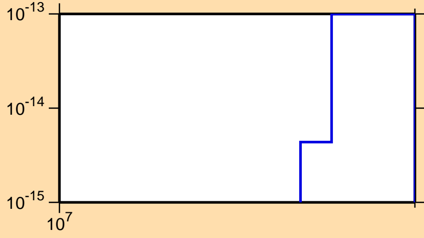
\sigma vs. E for ^{229}\text{Np}(n,\text{pd})
