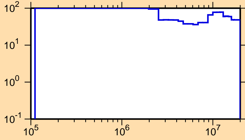
\Delta\sigma/\sigma vs. E for ^{229}\text{Np}(n,ncont.)
