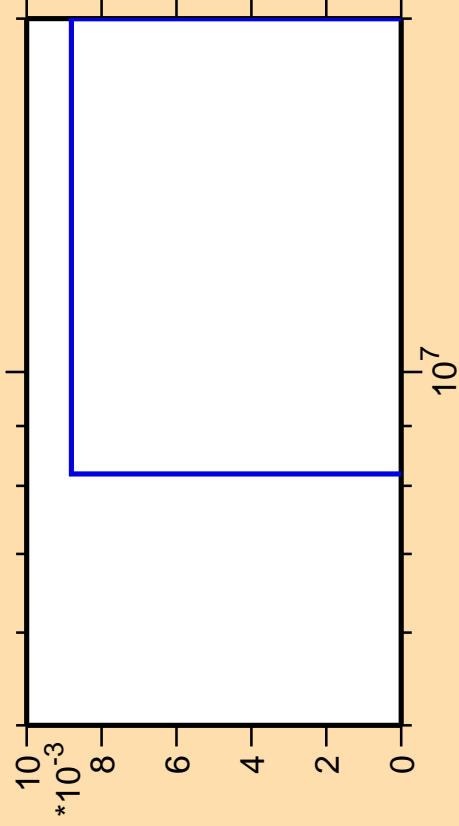
\Delta\sigma/\sigma vs. E for ^{229}\text{Np}(n,pd)
