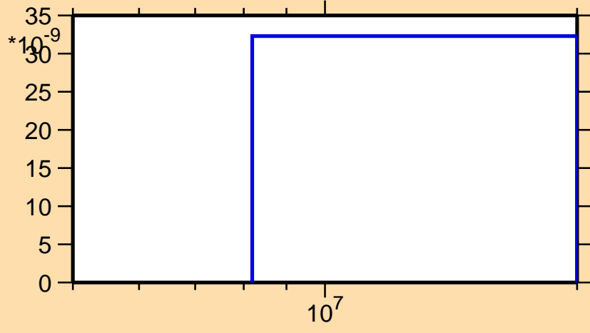
\sigma vs. E for ^{229}\text{Np}(n,nd)
