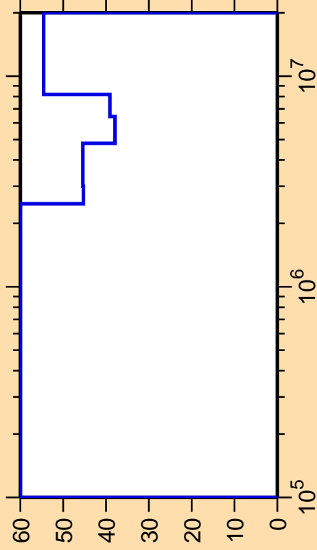
\Delta\sigma/\sigma vs. E for ^{229}\text{Np}(n,\text{inel.})
