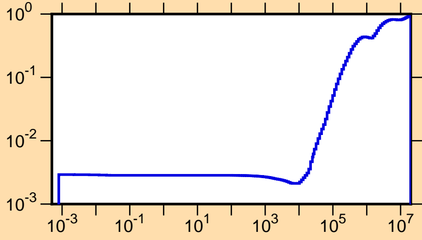
\mu vs. E for ^{230}\text{Np}(\text{mt251})
