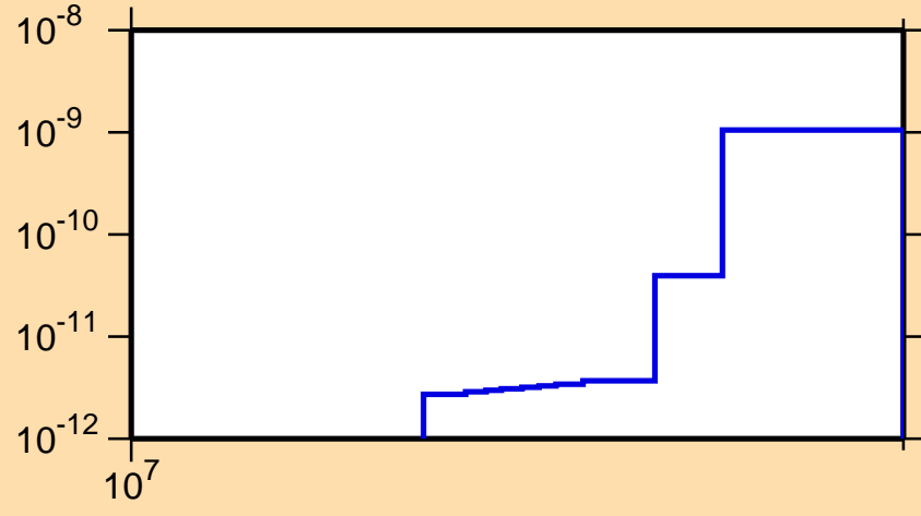
\sigma vs. E for ^{230}\text{Np}(n,3n\alpha)
