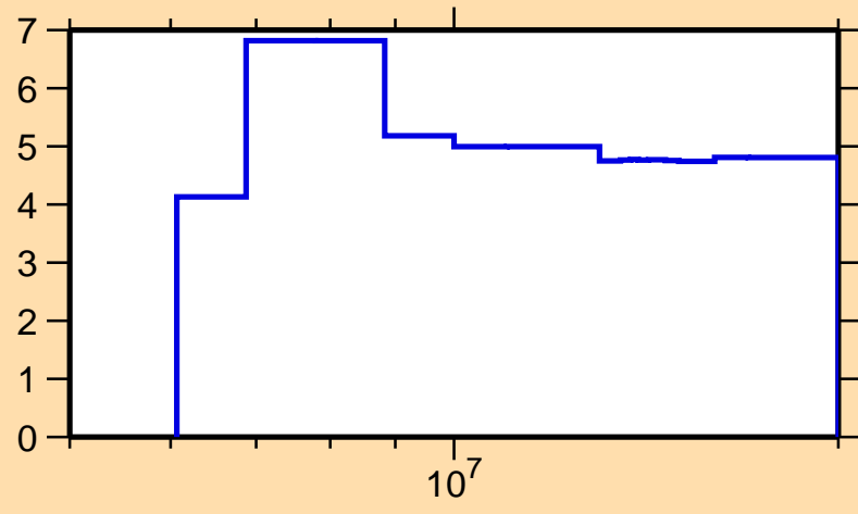
\Delta\sigma/\sigma vs. E for ^{230}\text{Np}(n,\text{nonel.})
