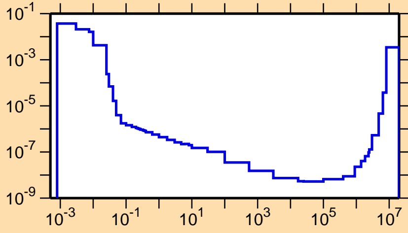
\sigma vs. E for ^{230}\text{Np}(n,\alpha)
