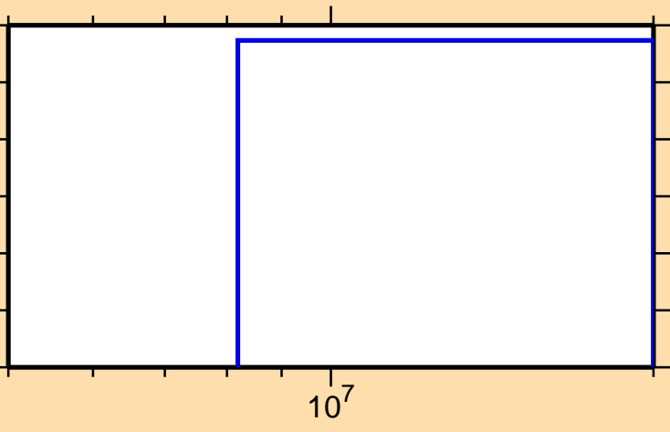
\sigma vs. E for ^{230}\text{Np}(n,\text{He}3)
