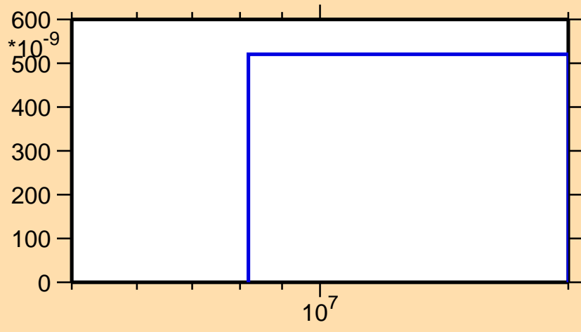
\sigma vs. E for ^{230}\text{Np}(n,nd)
