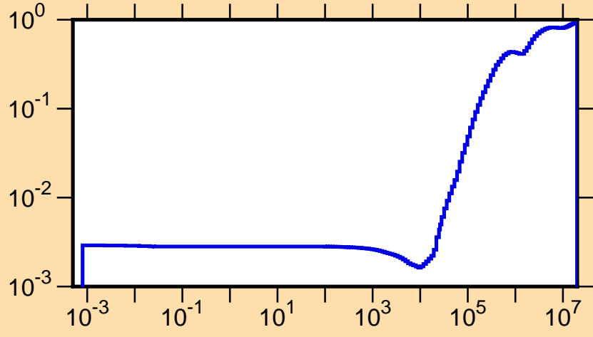
\mu vs. E for ^{231}\text{Np}(\text{mt251})
