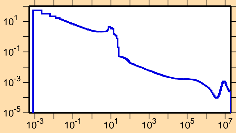
\sigma vs. E for ^{231}\text{Np}(n,\gamma)
