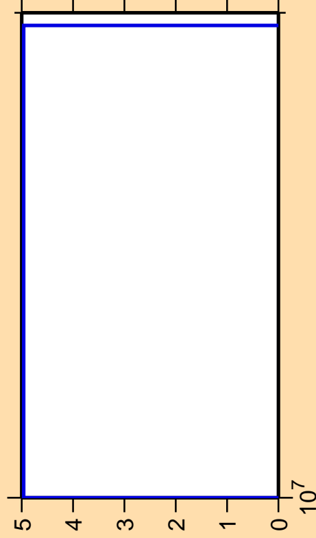
\Delta\sigma/\sigma vs. E for ^{231}\text{Np}(n,p\alpha)
