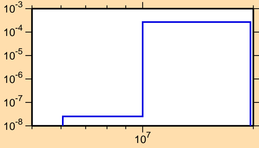
\sigma vs. E for ^{231}\text{Np}(n,np)
