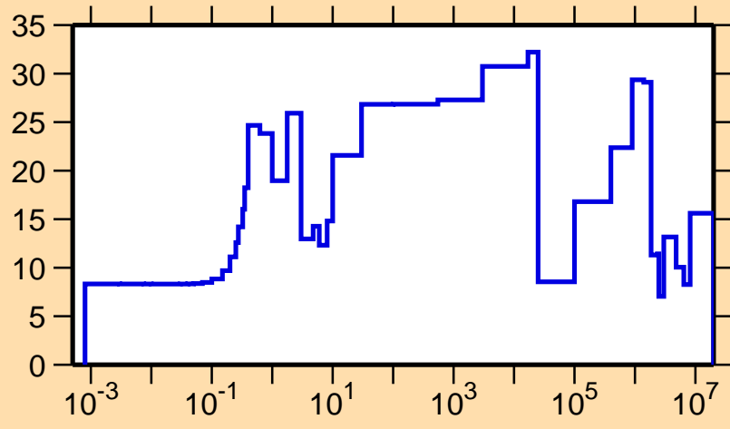
\Delta\sigma/\sigma vs. E for ^{231}\text{Np}(n,f)
