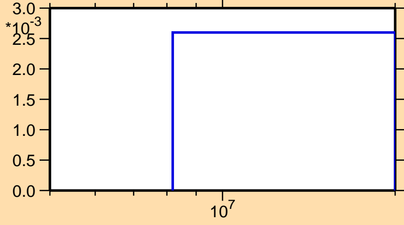
\sigma vs. E for ^{231}\text{Np}(n,3n)
