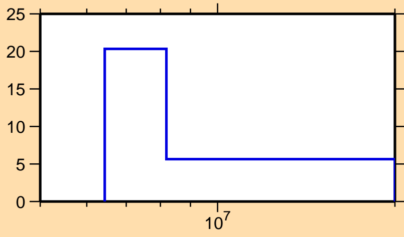
\Delta\sigma/\sigma vs. E for ^{231}\text{Np}(n,\text{tot.})
