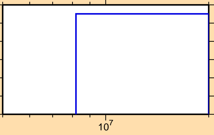
\sigma vs. E for ^{231}\text{Np}(n,2n\alpha)
