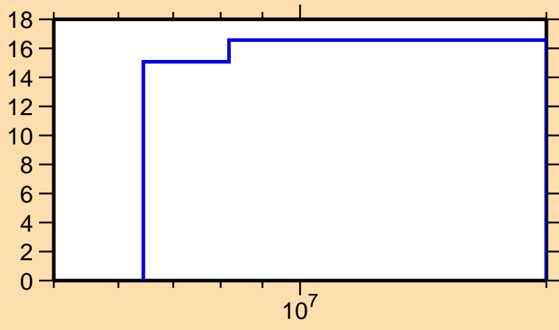
\Delta\sigma/\sigma vs. E for ^{231}\text{Np}(n,\text{inel.})
