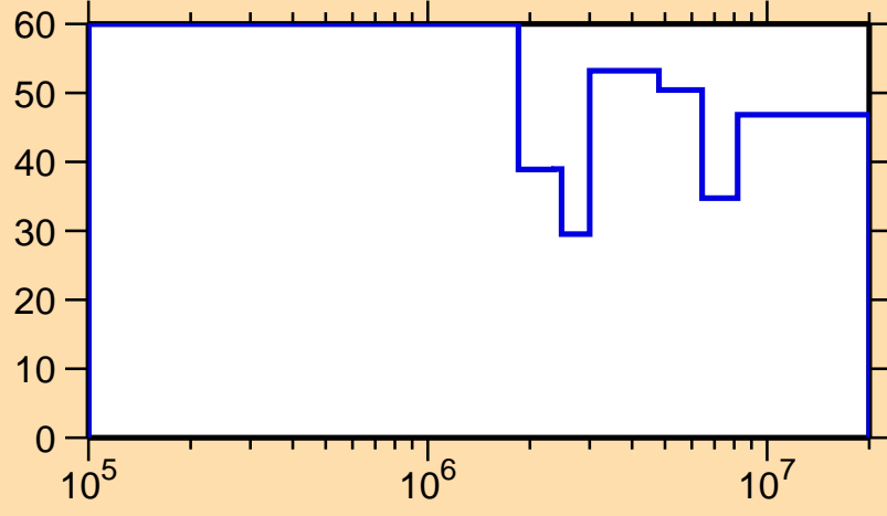
\Delta\sigma/\sigma vs. E for ^{231}\text{Np}(n,n_1)
