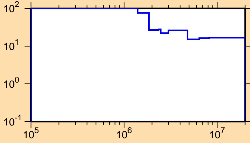
\Delta\sigma/\sigma vs. E for ^{231}\text{Np}(n,n\text{cont.})
