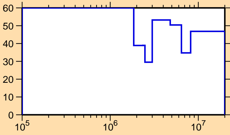
\Delta\sigma/\sigma vs. E for ^{231}\text{Np}(n,n_1)
