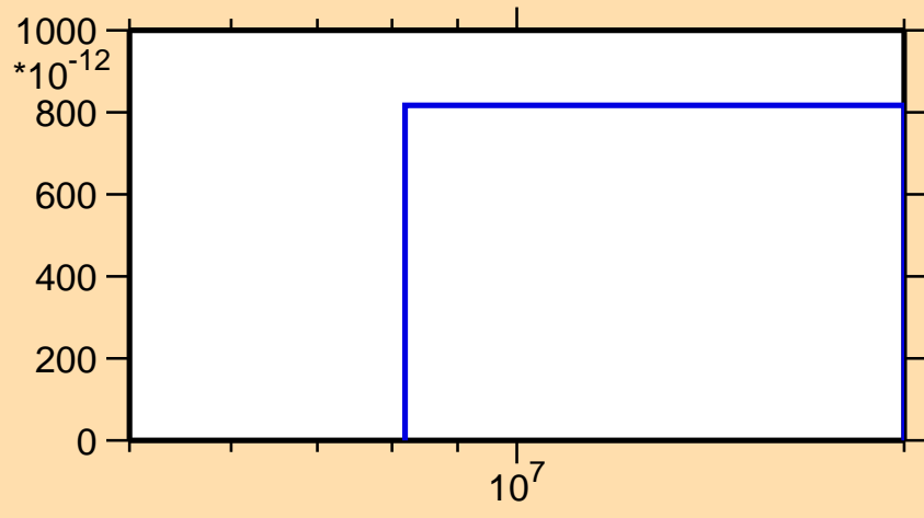
\sigma vs. E for ^{231}\text{Np}(n,2np)
