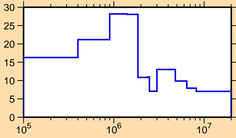
\Delta\sigma/\sigma vs. E for ^{231}\text{Np}(n,\text{nonel.})
