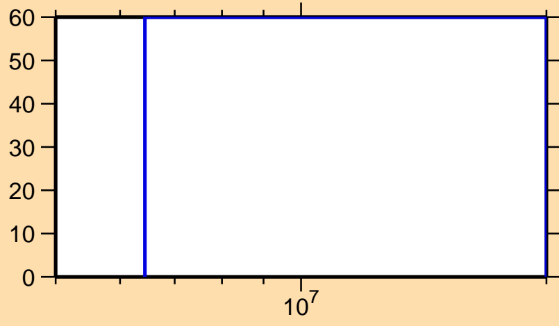
\Delta\sigma/\sigma vs. E for ^{231}\text{Np}(n,2n)
