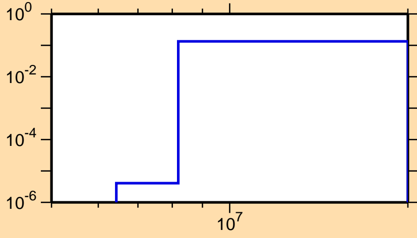
\sigma vs. E for ^{231}\text{Np}(n,2n)
