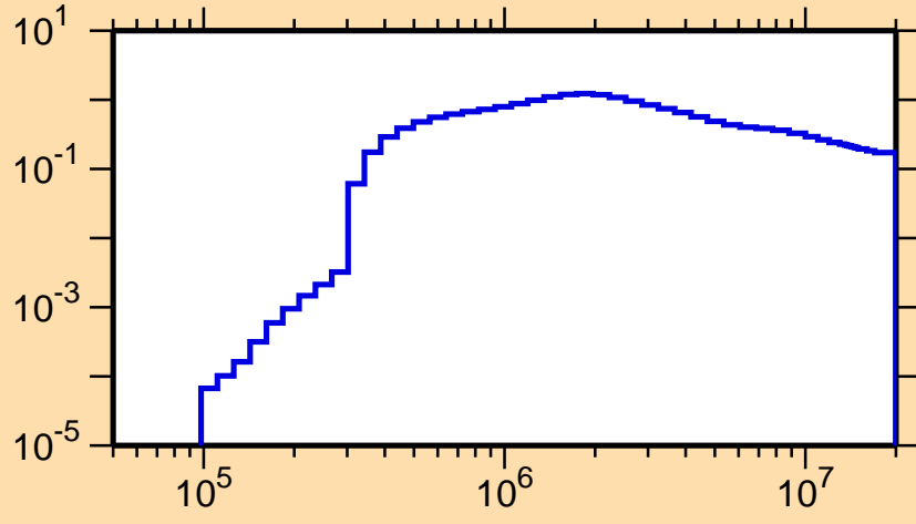
\sigma vs. E for ^{232}\text{Np}(n,\text{inel.})
