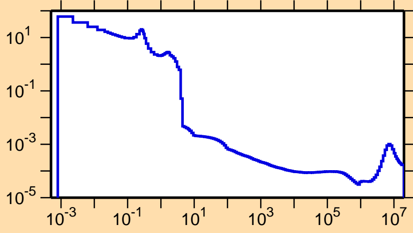
\sigma vs. E for ^{232}\text{Np}(n,\gamma)
