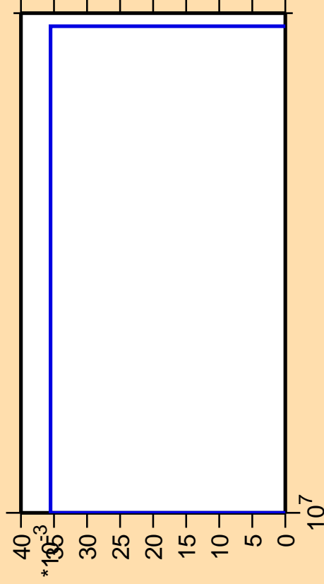
\Delta\sigma/\sigma vs. E for ^{232}\text{Np} (mt 45)
