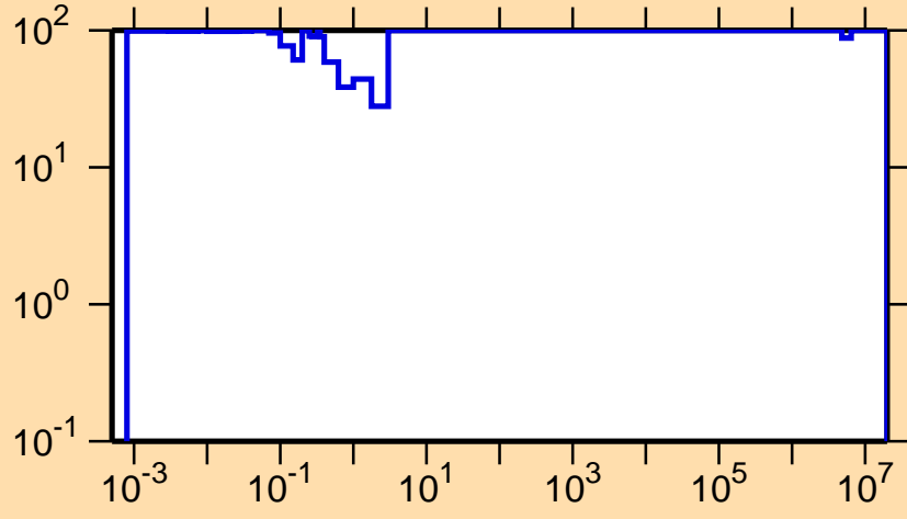
\Delta\sigma/\sigma vs. E for ^{232}\text{Np}(n,\gamma)
