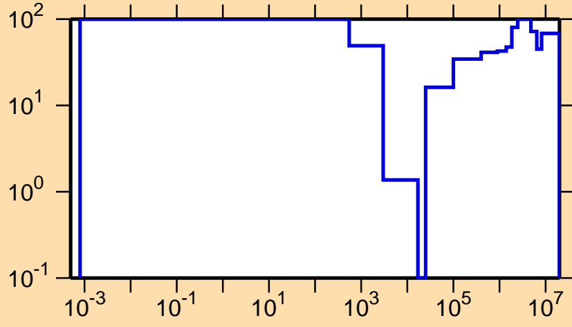
\Delta\sigma/\sigma vs. E for ^{232}\text{Np}(n,p)
