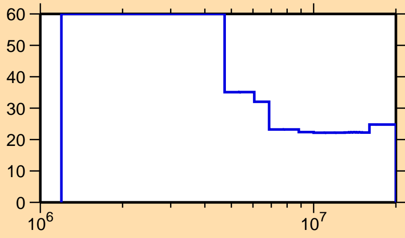
\Delta\sigma/\sigma vs. E for ^{233}\text{Np}(n,ncont.)
