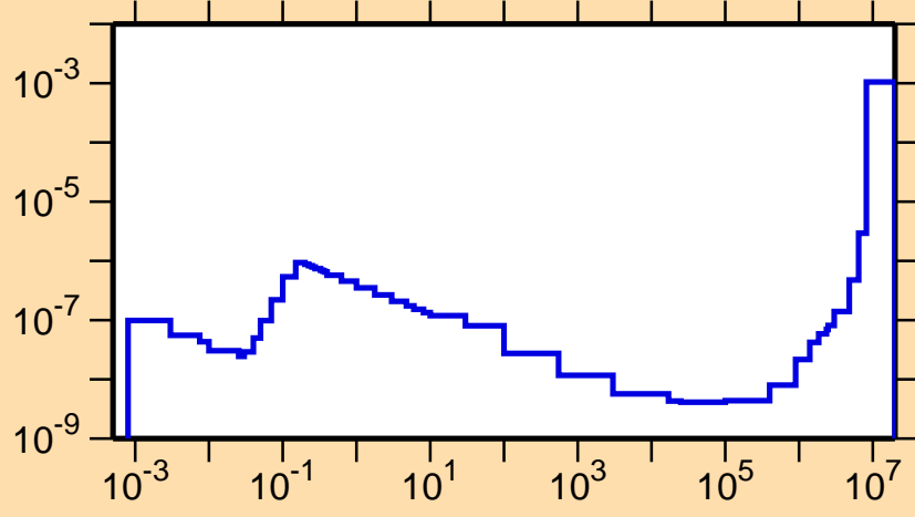
\sigma vs. E for ^{233}\text{Np}(n,\alpha)
