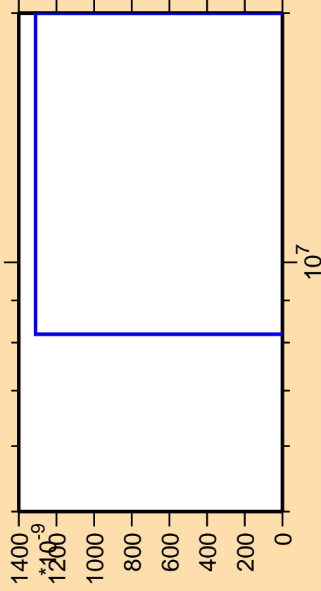
\Delta\sigma/\sigma vs. E for ^{233}\text{Np}(\text{mt } 11)
