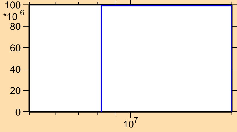
\sigma vs. E for ^{233}\text{Np}(n,3n)
