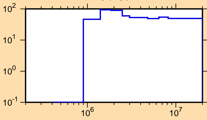
\Delta\sigma/\sigma vs. E for ^{233}\text{Np}(n,p)
