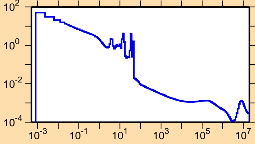
\sigma vs. E for ^{234}\text{Np}(n,\gamma)
