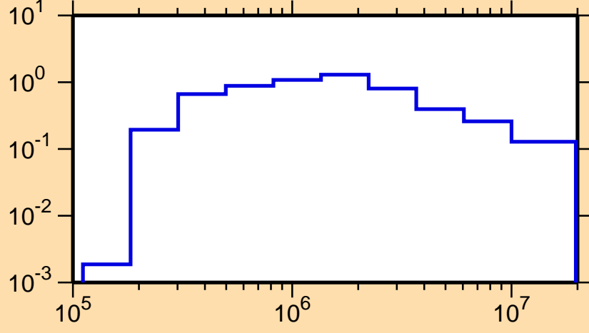
\sigma vs. E for ^{234}\text{Np}(n,n_1)
