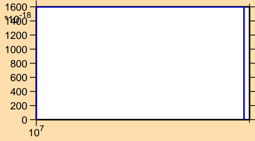
\sigma vs. E for ^{234}\text{Np}(n,3n\alpha)
