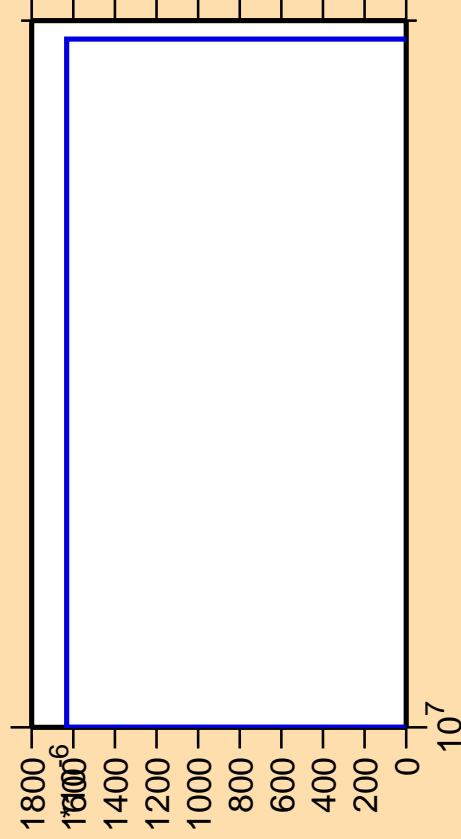
\Delta\sigma/\sigma vs. E for ^{234}\text{Np}(n,3n\alpha)
