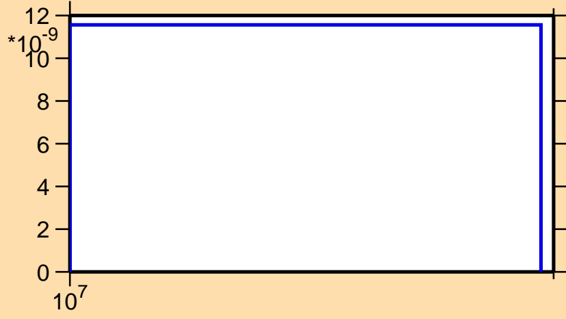
\sigma vs. E for ^{234}\text{Np}(n,2np)
