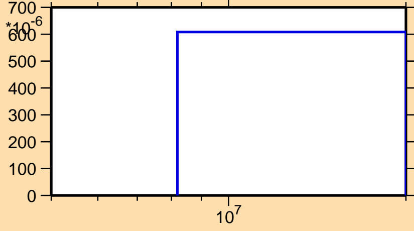
\sigma vs. E for ^{234}\text{Np}(n,3n)
