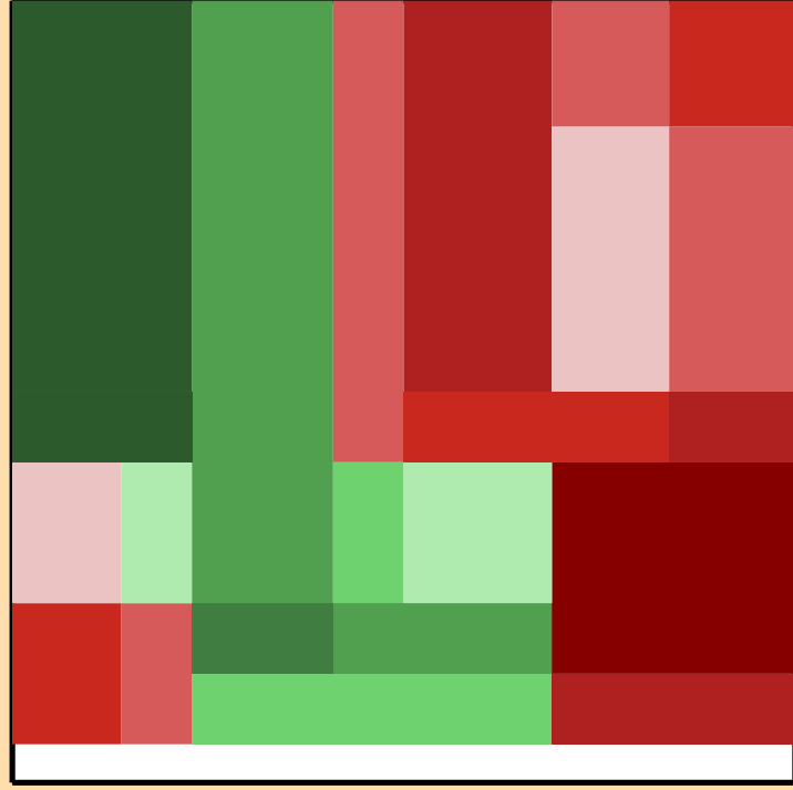
\Delta\sigma/\sigma vs. E for ^{236}\text{Np}(n,\text{el.})
