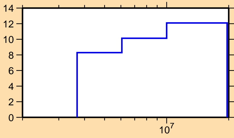
\Delta\sigma/\sigma vs. E for ^{2336}\text{Np}(n,\text{nonel.})
