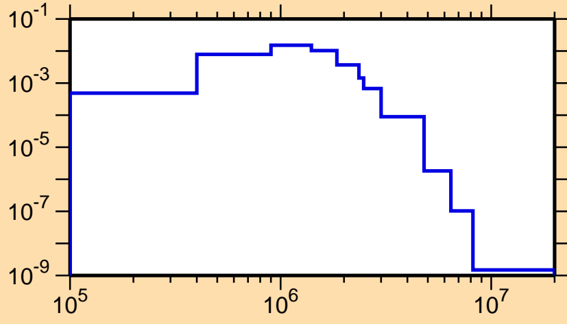
\sigma vs. E for ^{236}\text{Np}(n,n_4)
