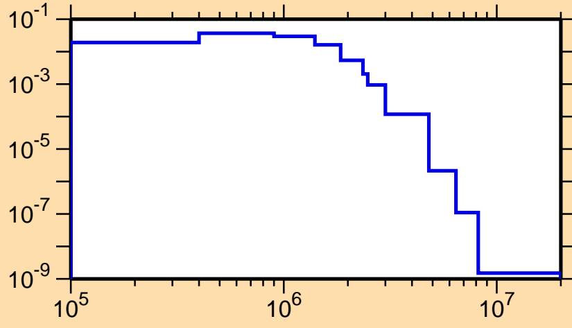
\sigma vs. E for ^{236}\text{Np}(n,n_3)
