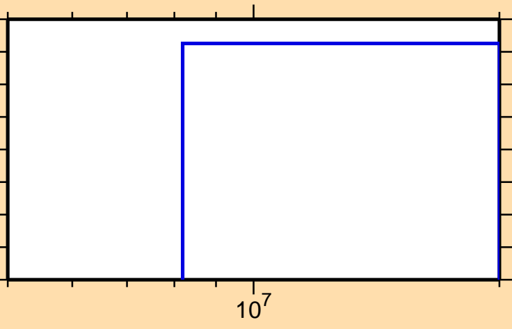
\sigma vs. E for ^{236}\text{Np}(n,2np)
