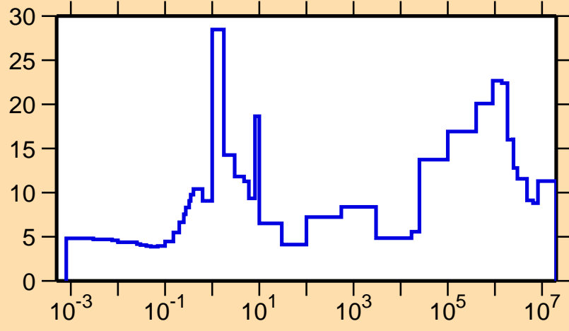
\Delta\sigma/\sigma vs. E for ^{236}\text{Np}(n,tot.)
