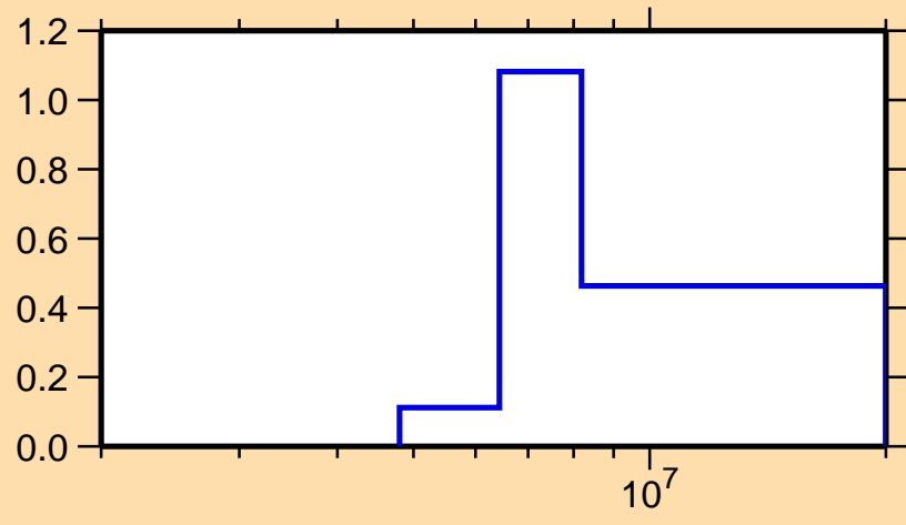
\sigma vs. E for ^{236}\text{Np}(n,2n)
