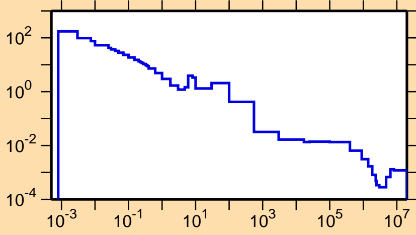
\sigma vs. E for ^{236}\text{Np}(n,\gamma)
