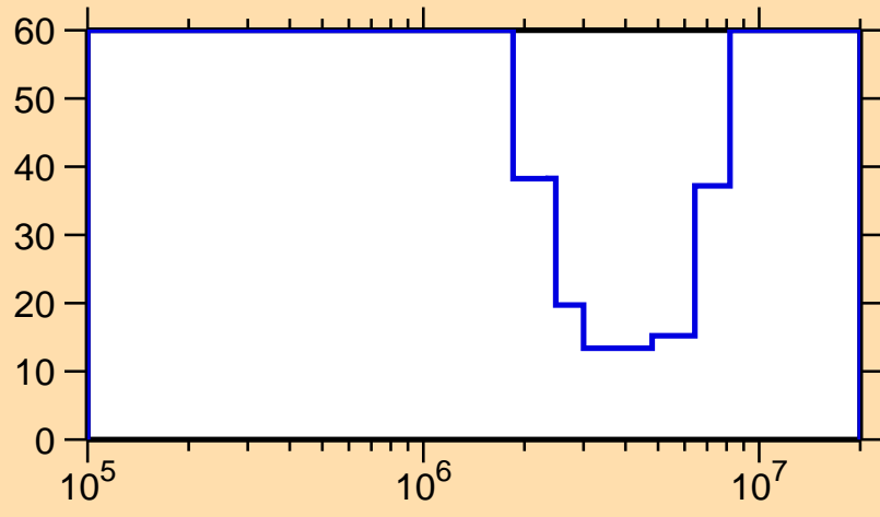
\Delta\sigma/\sigma vs. E for ^{236}\text{Np}(n,n\text{cont.})
