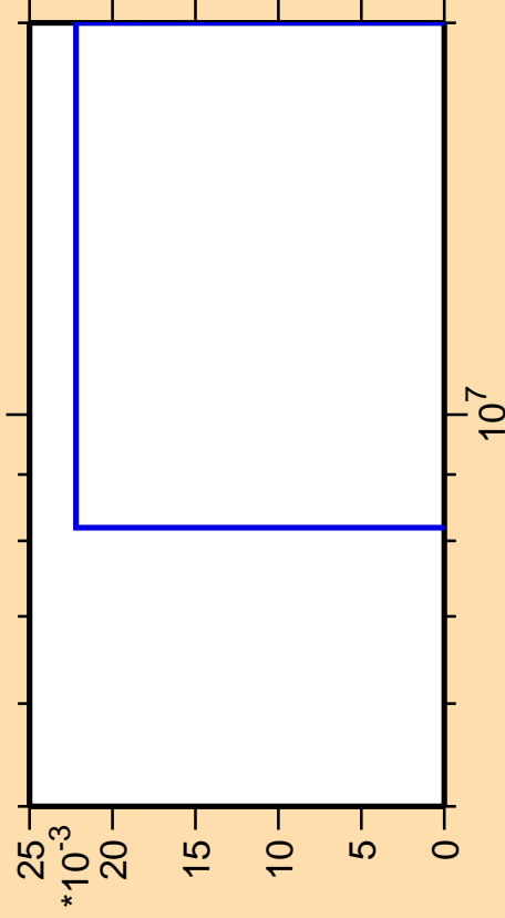
\Delta\sigma/\sigma vs. E for ^{236}\text{Np}(\text{mt } 11)
