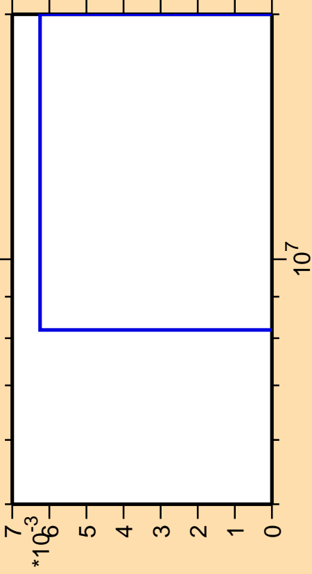
\Delta\sigma/\sigma vs. E for ^{236}\text{Np}(n,3n\alpha)
