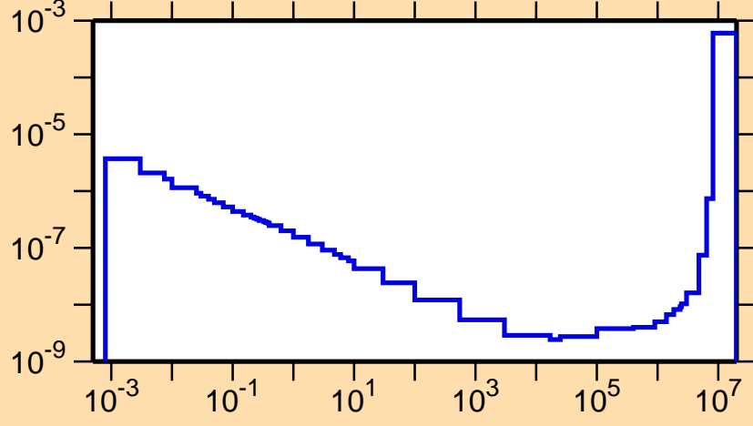
\sigma vs. E for ^{236}\text{Np}(n,\alpha)
