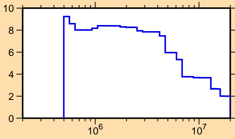
\Delta\sigma/\sigma vs. E for ^{237}\text{Np}(n,n\text{nonel.})
