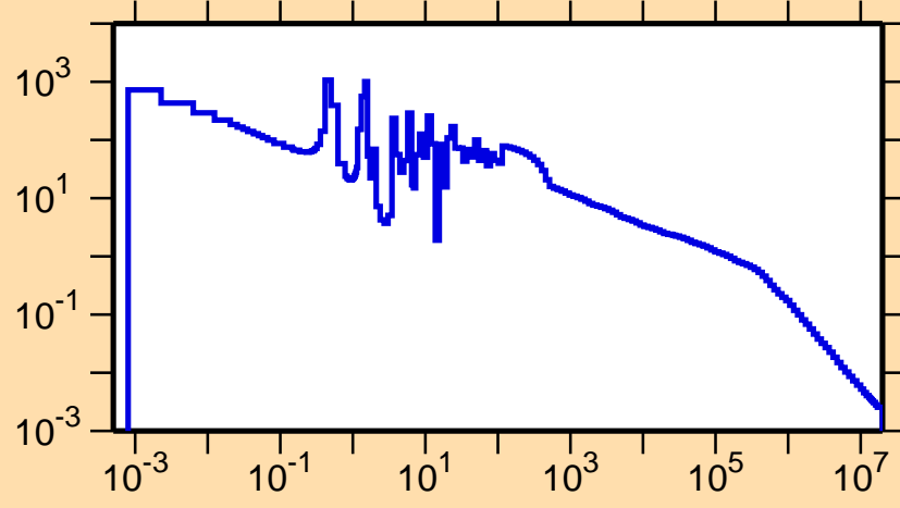
\sigma vs. E for ^{237}\text{Np}(n,\gamma)
