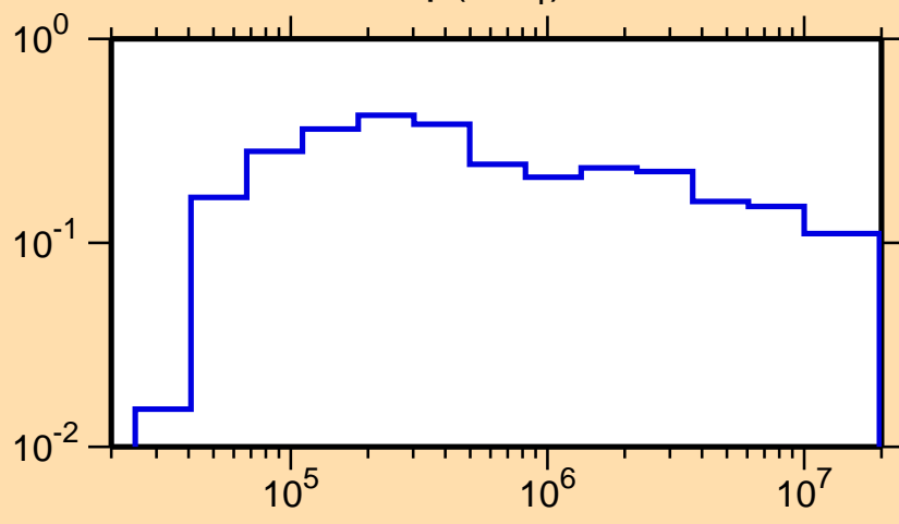
\sigma vs. E for ^{237}\text{Np}(n,n_1)
