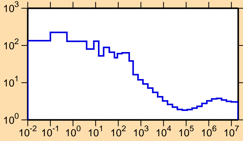
\sigma vs. E for ^{237}\text{Np}(n,\text{nonel.})
