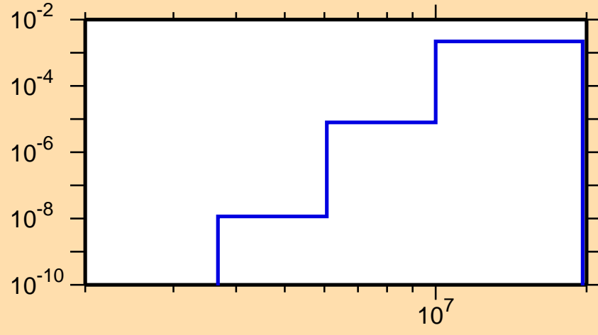
\sigma vs. E for ^{237}\text{Np}(n,p)
