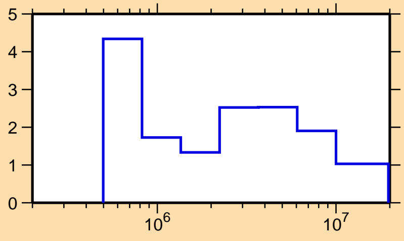
\Delta\sigma/\sigma vs. E for ^{237}\text{Np}(n,f)
