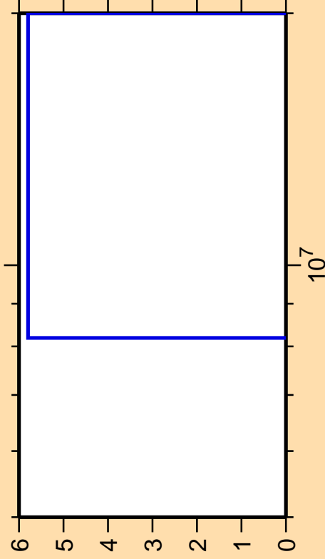
\Delta\sigma/\sigma vs. E for ^{237}\text{Np}(n,nd)
