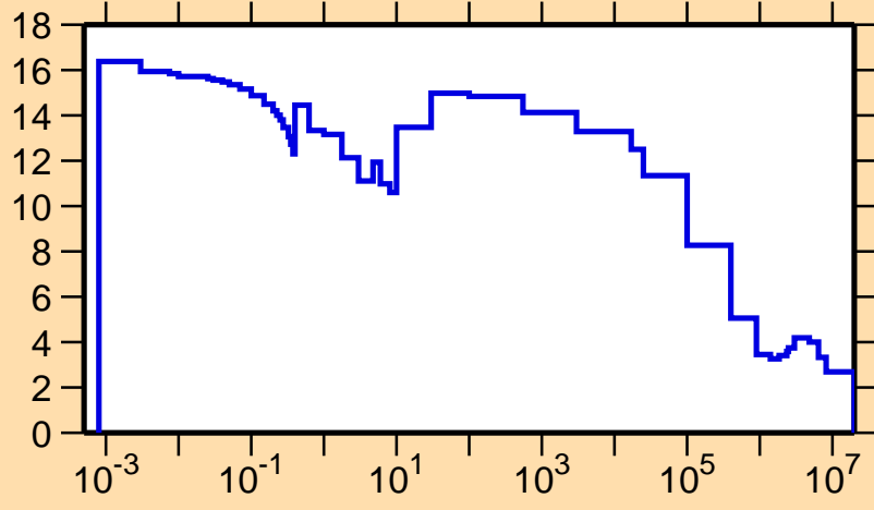
\sigma vs. E for ^{237}\text{Np}(n,\text{el.})
