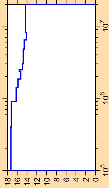
\Delta\sigma/\sigma vs. E for ^{237}\text{Np}(n,n_4)
