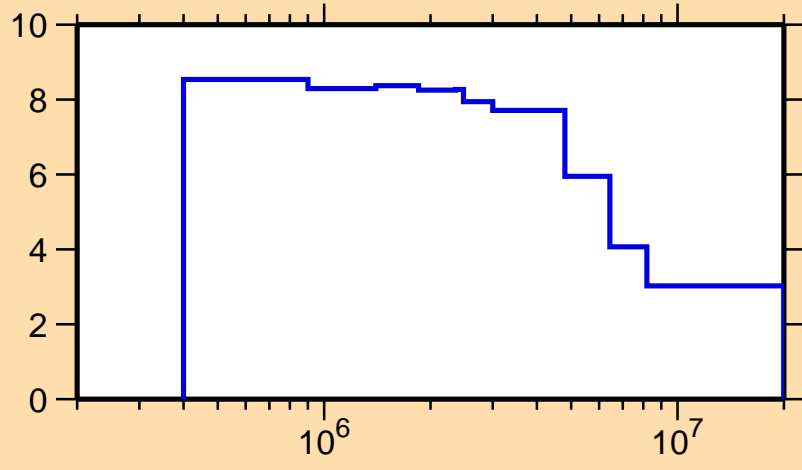
\Delta\sigma/\sigma vs. E for ^{237}\text{Np}(n,n\text{onel.})
