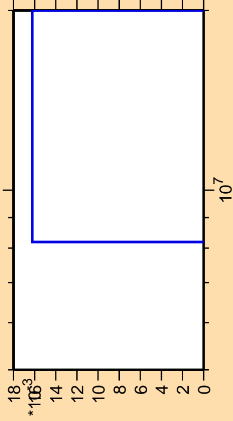
\Delta\sigma/\sigma vs. E for ^{237}\text{Np}(n,3n\alpha)
