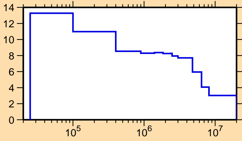
\Delta\sigma/\sigma vs. E for ^{237}\text{Np}(n,\text{nonel.})
