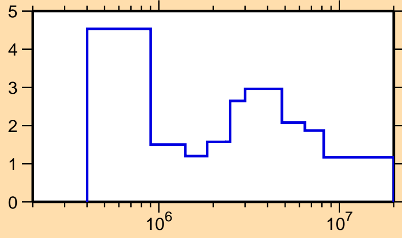
\Delta\sigma/\sigma vs. E for ^{237}\text{Np}(n,f)
