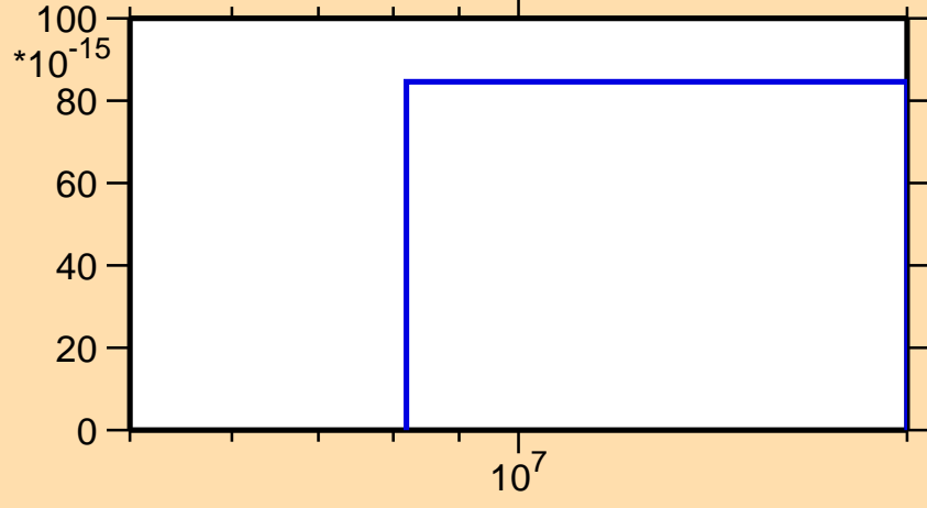
\sigma vs. E for ^{237}\text{Np}(n,3n\alpha)
