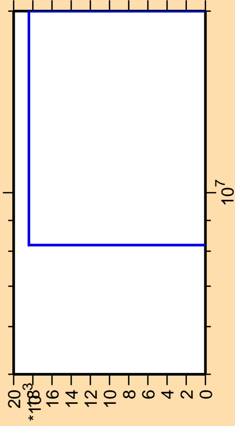
\Delta\sigma/\sigma vs. E for ^{237}\text{Np}(n,\text{He}3)
