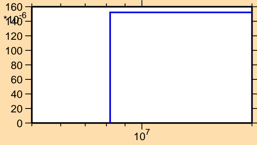
\sigma vs. E for ^{237}\text{Np}(n,np)
