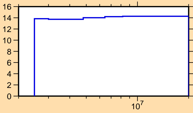
\Delta\sigma/\sigma vs. E for ^{237}\text{Np}(n,n_1)
