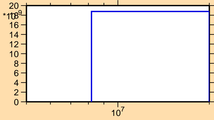
\sigma vs. E for ^{237}\text{Np}(n,nd)
