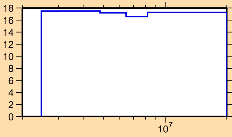
\Delta\sigma/\sigma vs. E for ^{237}\text{Np}(n,\gamma)
