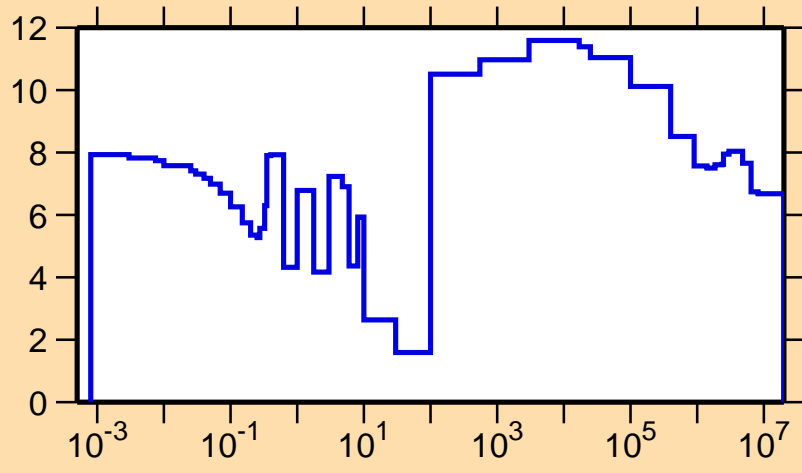
\Delta\sigma/\sigma vs. E for ^{237}\text{Np}(n,tot.)
