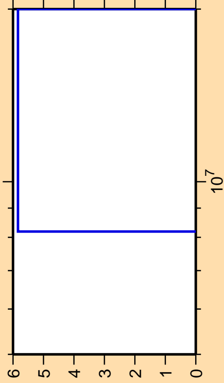
\Delta\sigma/\sigma vs. E for ^{237}\text{Np}(n,2np)
