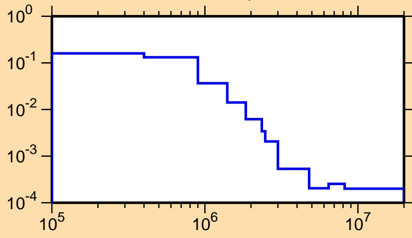
\sigma vs. E for ^{237}\text{Np}(n,n_4)
