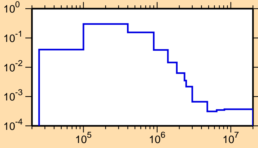
\sigma vs. E for ^{237}\text{Np}(n,n_2)
