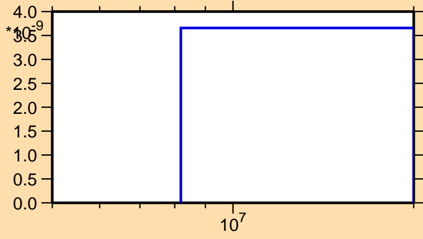
\sigma vs. E for ^{237}\text{Np}(n,2n\alpha)
