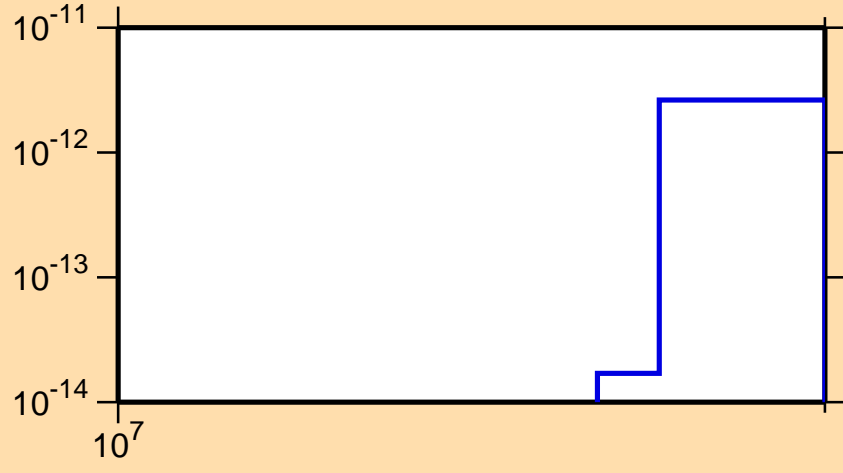
\sigma vs. E for ^{238}\text{Np}(n,3n\alpha)
