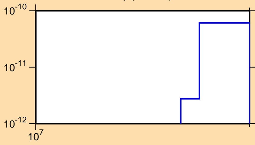
\sigma vs. E for ^{238}\text{Np}(n,\text{He3})
