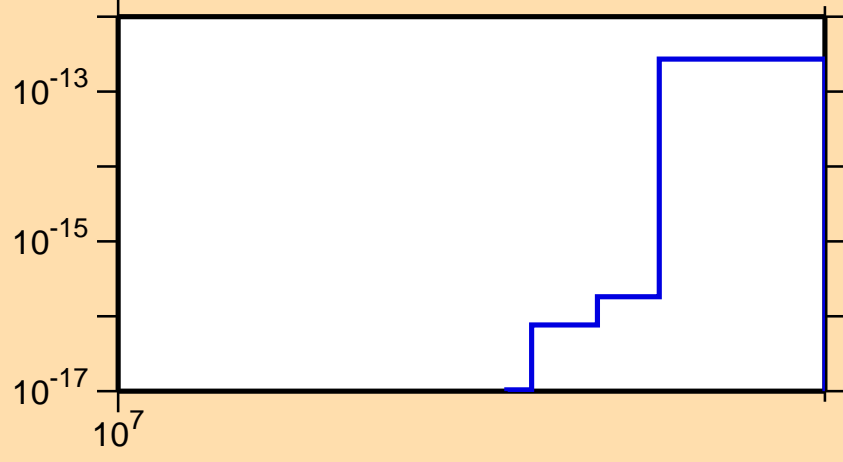
\sigma vs. E for ^{238}\text{Np} (mt 11)
