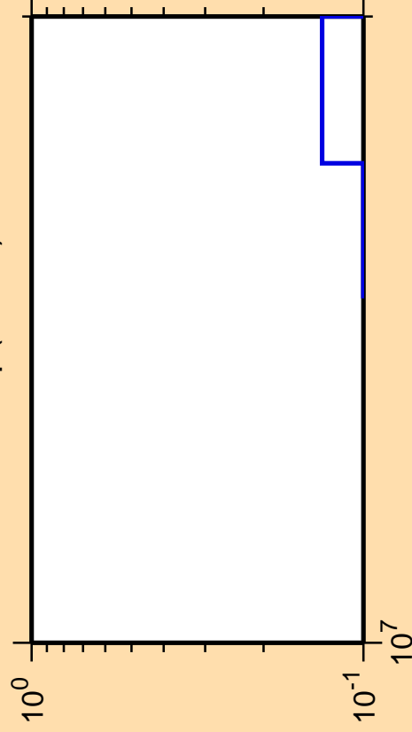
\Delta\sigma/\sigma vs. E for ^{238}\text{Np} (mt 11)
