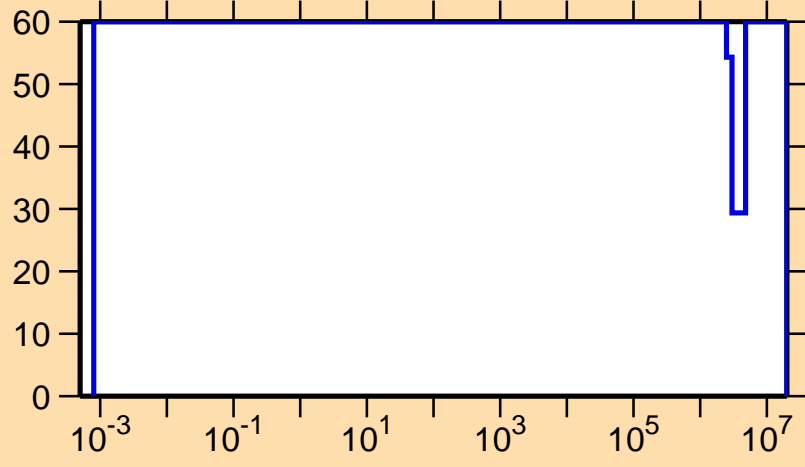
\Delta\sigma/\sigma vs. E for ^{238}\text{Np}(n,\gamma)
