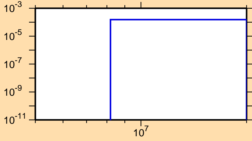
\sigma vs. E for ^{238}\text{Np}(n,d)
