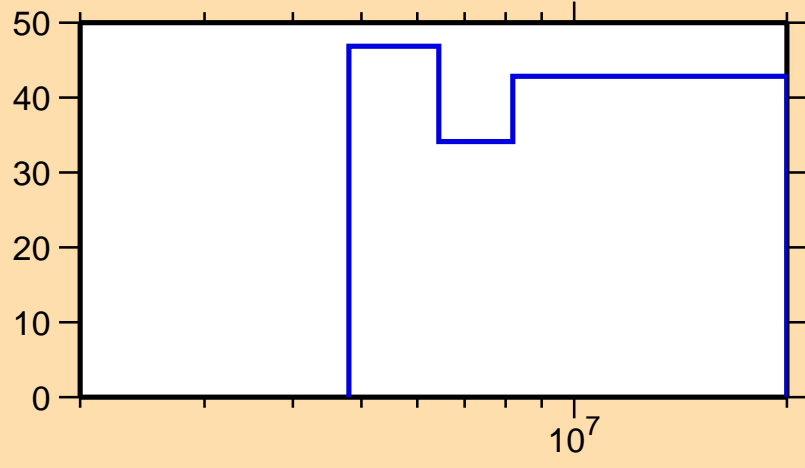
\Delta\sigma/\sigma vs. E for ^{238}\text{Np}(n,\text{inel.})
