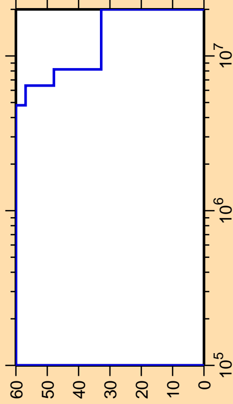
\Delta\sigma/\sigma vs. E for ^{238}\text{Np}(n,n_4)
