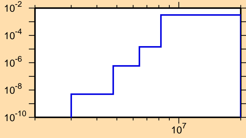
\sigma vs. E for ^{238}\text{Np}(n,p)
