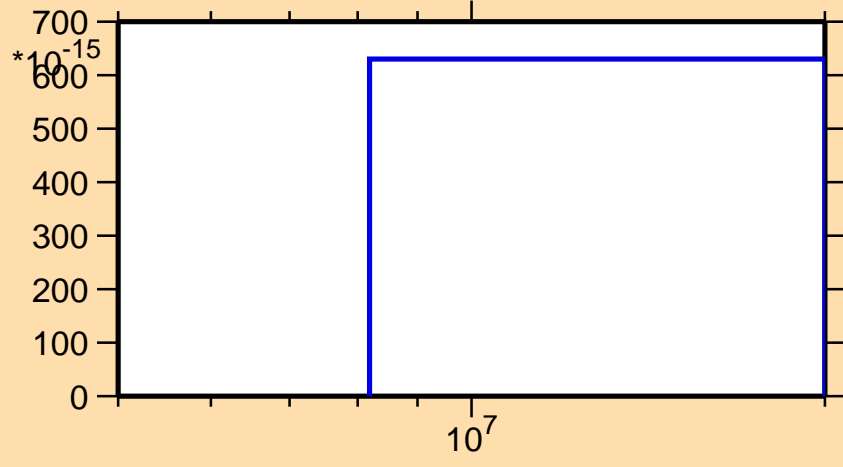
\sigma vs. E for ^{238}\text{Np}(n,\text{He3})
