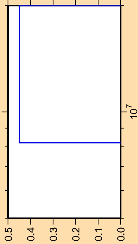
\Delta\sigma/\sigma vs. E for ^{238}\text{Np}(n,\text{He3})
