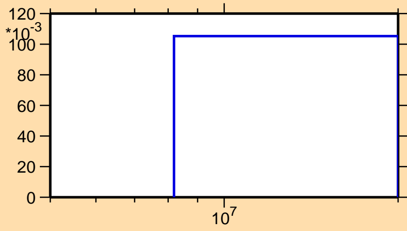
\sigma vs. E for ^{238}\text{Np}(n,3n)
