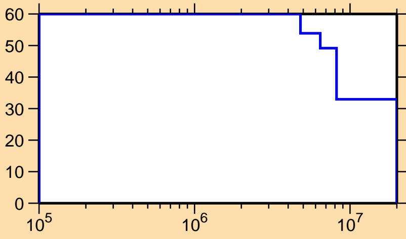
\Delta\sigma/\sigma vs. E for ^{238}\text{Np}(n,n_1)
