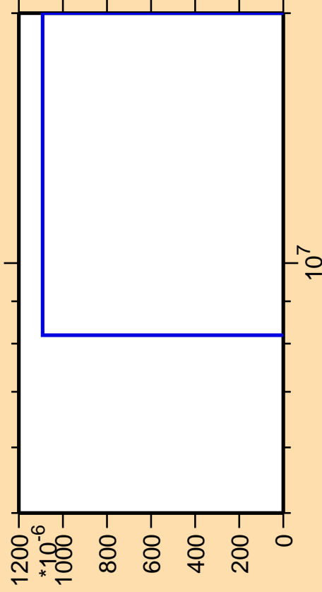
\Delta\sigma/\sigma vs. E for ^{238}\text{Np}(\text{mt } 11)
