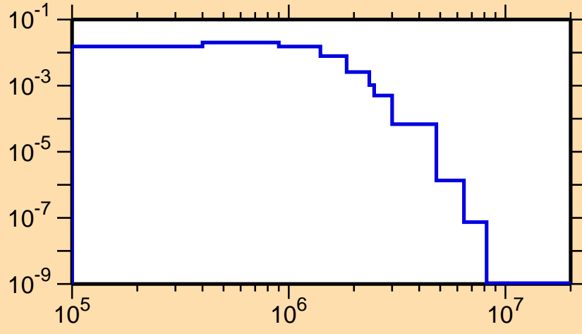
\sigma vs. E for ^{238}\text{Np}(n,n_4)
