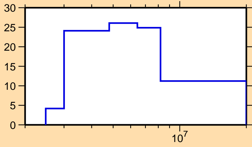
\Delta\sigma/\sigma vs. E for ^{238}\text{Np}(n,p)
