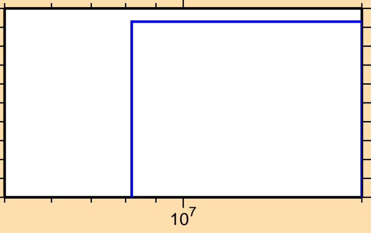
\sigma vs. E for ^{238}\text{Np}(n,nd)
