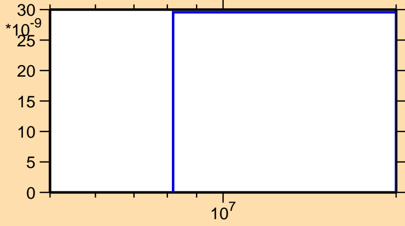
\sigma vs. E for ^{238}\text{Np}(n,2np)
