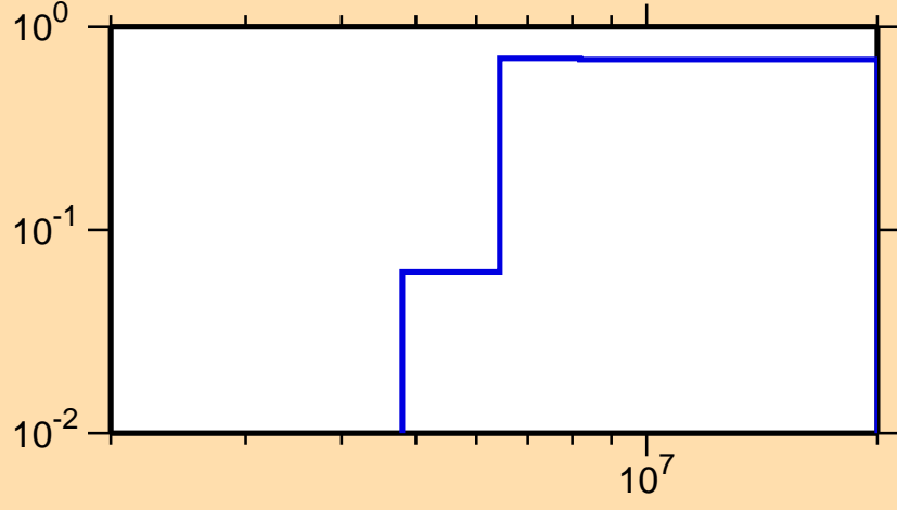
\sigma vs. E for ^{238}\text{Np}(n,2n)
