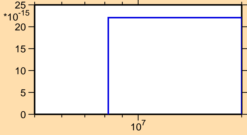
\sigma vs. E for ^{238}\text{Np}(n,3n\alpha)
