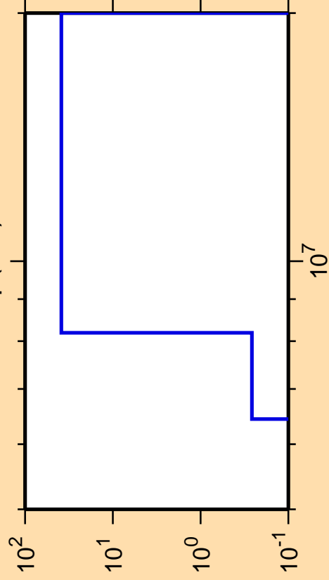
\Delta\sigma/\sigma vs. E for ^{238}\text{Np}(n,d)
