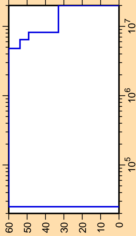
\Delta\sigma/\sigma vs. E for ^{238}\text{Np}(n,n_1)
