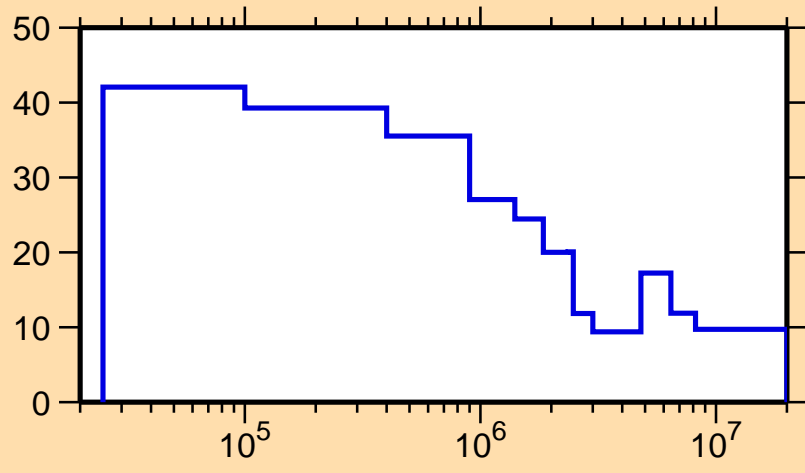
\Delta\sigma/\sigma vs. E for ^{238}\text{Np}(n,\text{nonel.})
