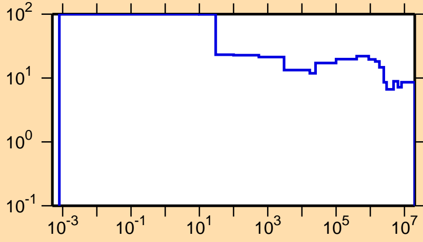
\Delta\sigma/\sigma vs. E for ^{238}\text{Np}(n,\text{tot.})
