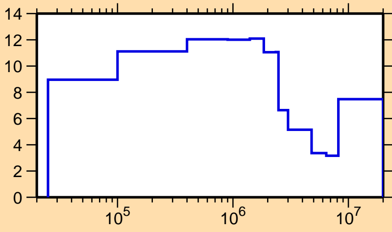
\Delta\sigma/\sigma vs. E for ^{238}\text{Np}(n,\text{el.})
