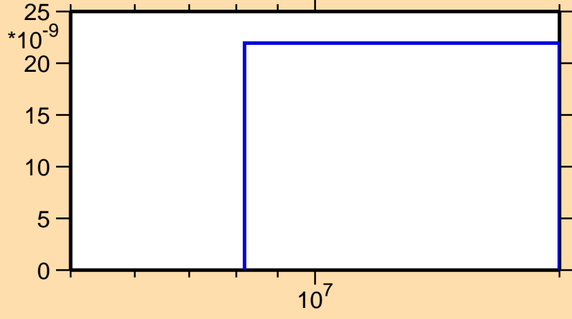
\sigma vs. E for ^{238}\text{Np}(n,2n\alpha)
