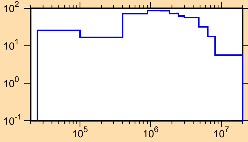
\Delta\sigma/\sigma vs. E for ^{238}\text{Np}(n,f)
