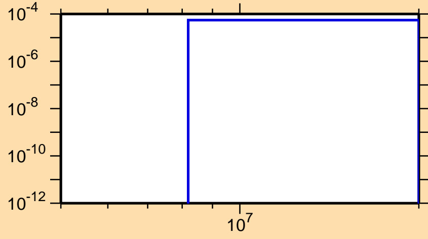
\sigma vs. E for ^{238}\text{Np}(n,t)
