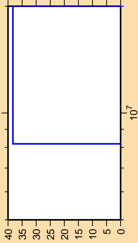
\Delta\sigma/\sigma vs. E for ^{238}\text{Np}(n,nd)
