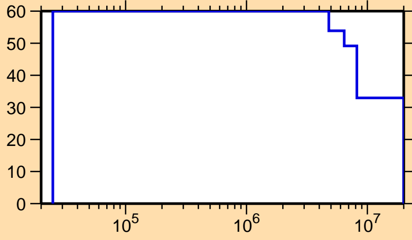
\Delta\sigma/\sigma vs. E for ^{238}\text{Np}(n,n_1)
