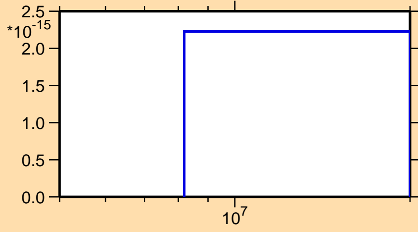
\sigma vs. E for ^{238}\text{Np}(\text{mt } 11)
