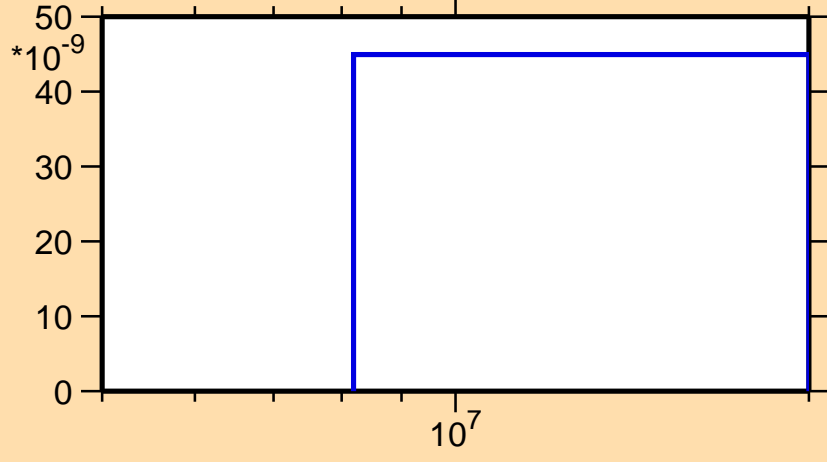
\sigma vs. E for ^{238}\text{Np}(n,nt)
