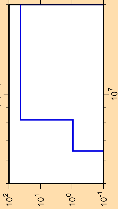
\Delta\sigma/\sigma vs. E for ^{238}\text{Np}(n,t)
