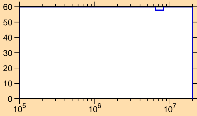
\Delta\sigma/\sigma vs. E for ^{238}\text{Np}(n,n\text{cont.})
