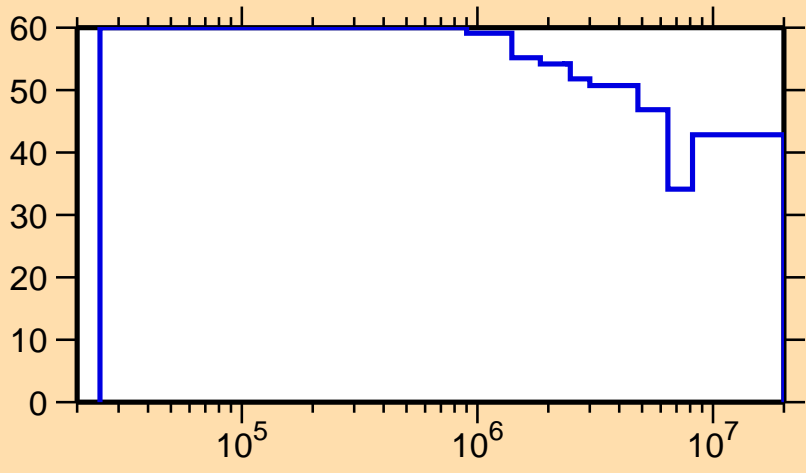
\Delta\sigma/\sigma vs. E for ^{238}\text{Np}(n,\text{inel.})
