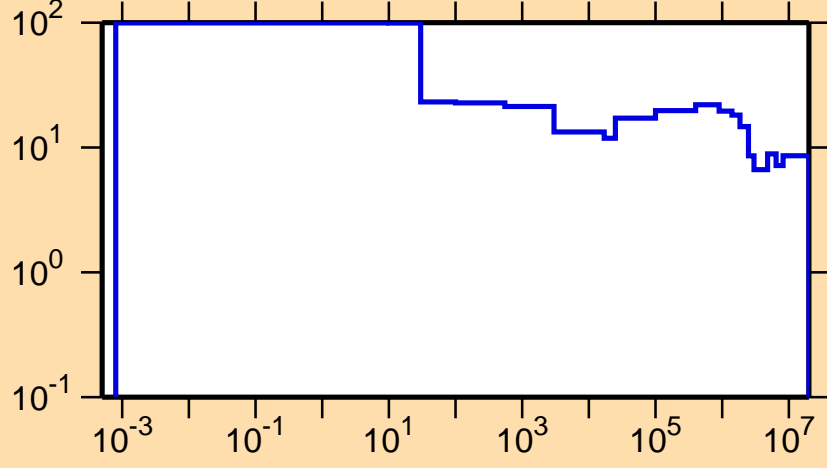
\Delta\sigma/\sigma vs. E for ^{238}\text{Np}(n,tot.)
