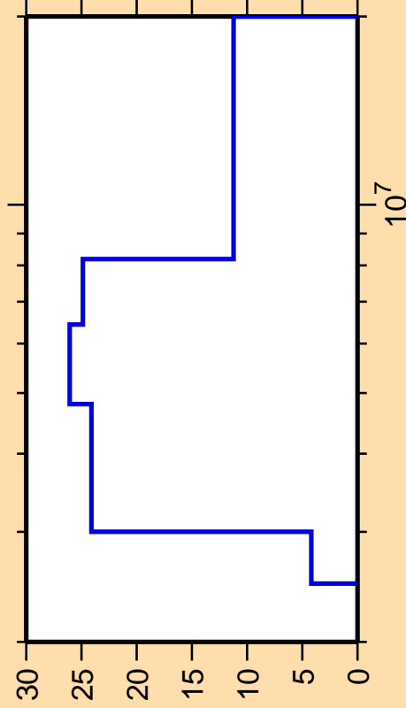
\Delta\sigma/\sigma vs. E for ^{238}\text{Np}(n,p)
