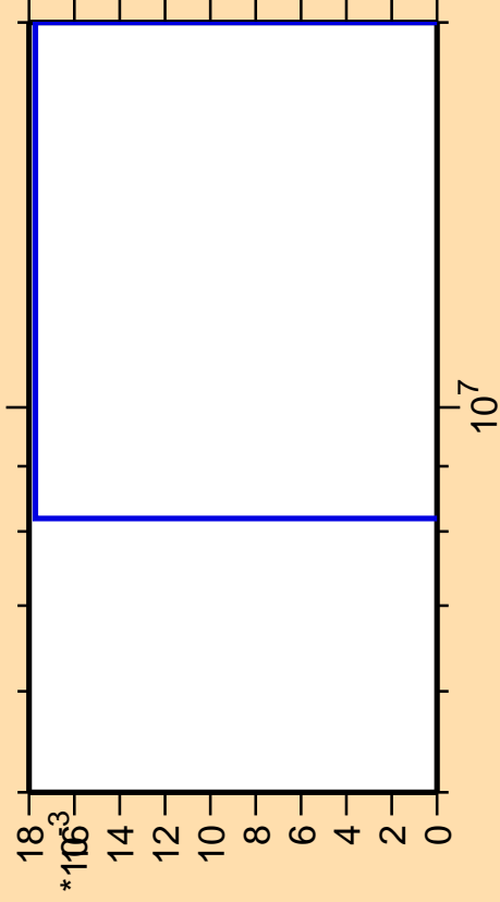
\Delta\sigma/\sigma vs. E for ^{238}\text{Np}(n,3n\alpha)
