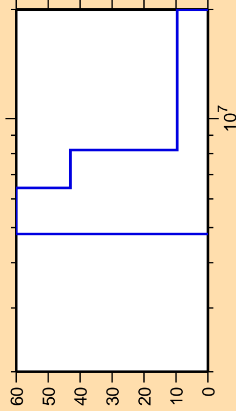
\Delta\sigma/\sigma vs. E for ^{238}\text{Np}(n,2n)
