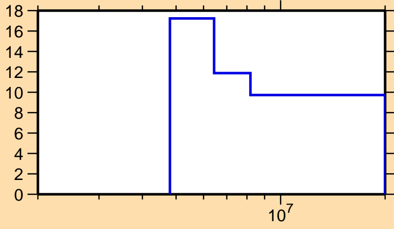
\Delta\sigma/\sigma vs. E for ^{238}\text{Np}(n,\text{nonel.})
