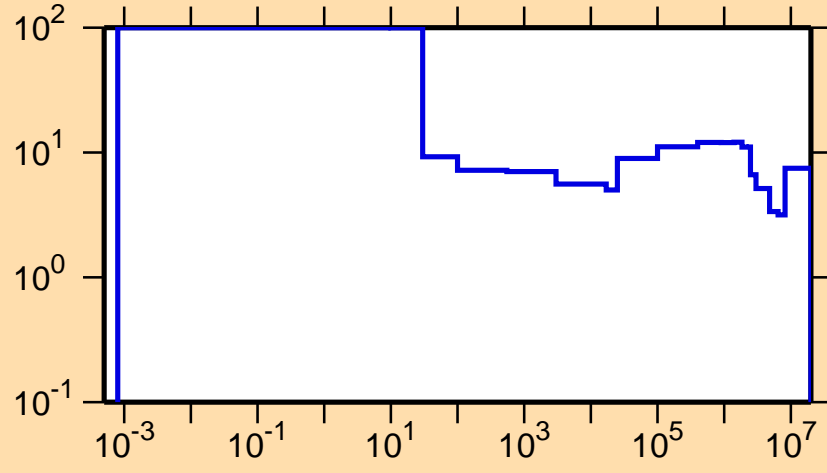
\Delta\sigma/\sigma vs. E for ^{238}\text{Np}(n,el.)
