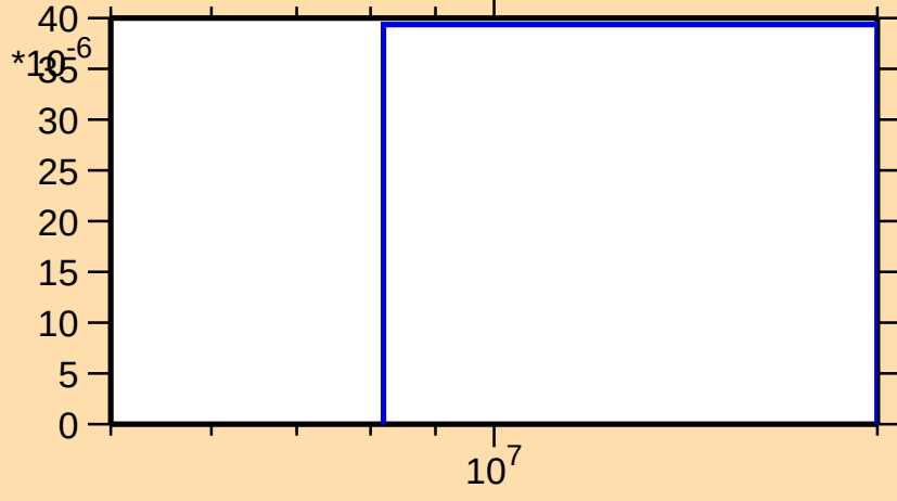
\sigma vs. E for ^{239}\text{Np}(n,t)
