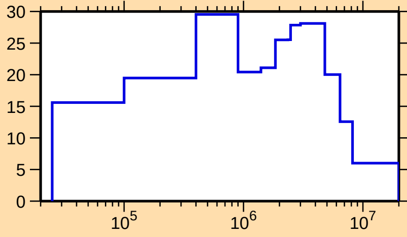
\Delta\sigma/\sigma vs. E for ^{239}\text{Np}(n,\text{tot.})
