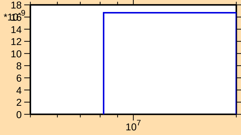
\sigma vs. E for ^{239}\text{Np}(n,\text{nd})
