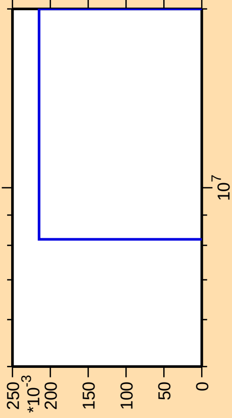
\Delta\sigma/\sigma vs. E for ^{239}\text{Np}(n,\text{He}3)
