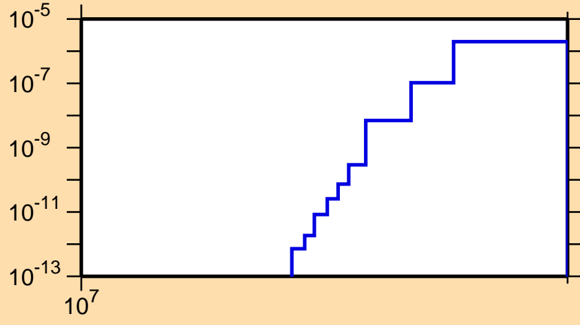
\sigma vs. E for ^{240}\text{Np}(n,2np)
