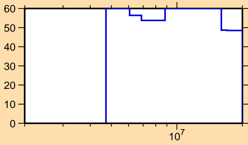
\Delta\sigma/\sigma vs. E for ^{240}\text{Np}(n,2n)
