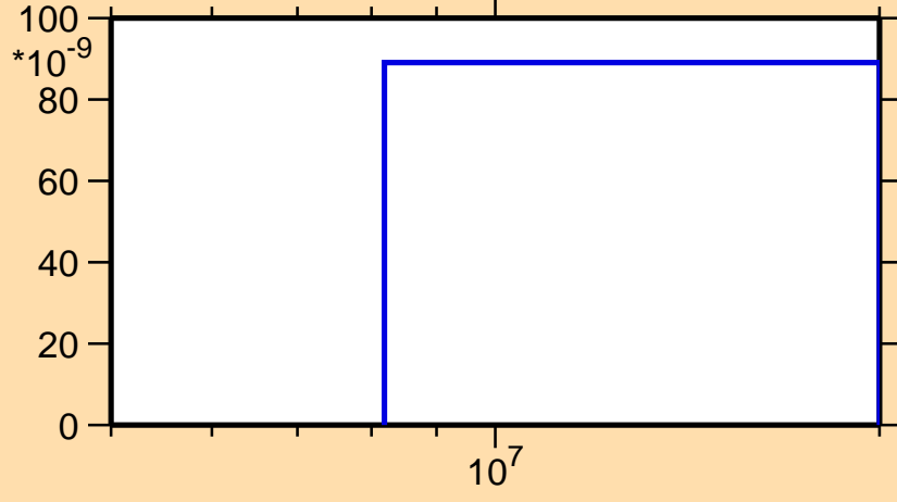
\sigma vs. E for ^{240}\text{Np}(n,nt)
