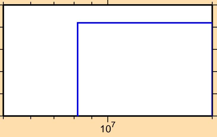
\sigma vs. E for ^{240}\text{Np}(n,2np)
