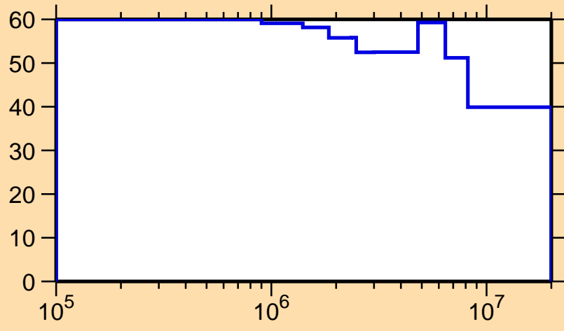
\Delta\sigma/\sigma vs. E for ^{240}\text{Np}(n,n\text{cont.})
