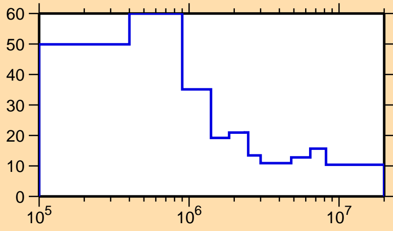
\Delta\sigma/\sigma vs. E for ^{240}\text{Np}(n,\text{el.})
