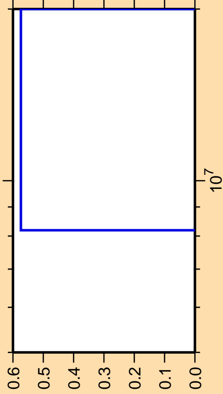
\Delta\sigma/\sigma vs. E for ^{240}\text{Np}(n,\text{He3})
