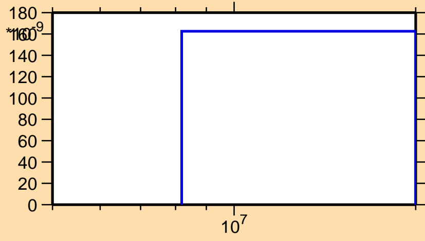
\sigma vs. E for ^{240}\text{Np}(n,nd)
