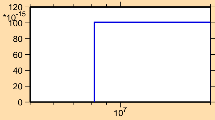
\sigma vs. E for ^{240}\text{Np}(n,\text{He3})
