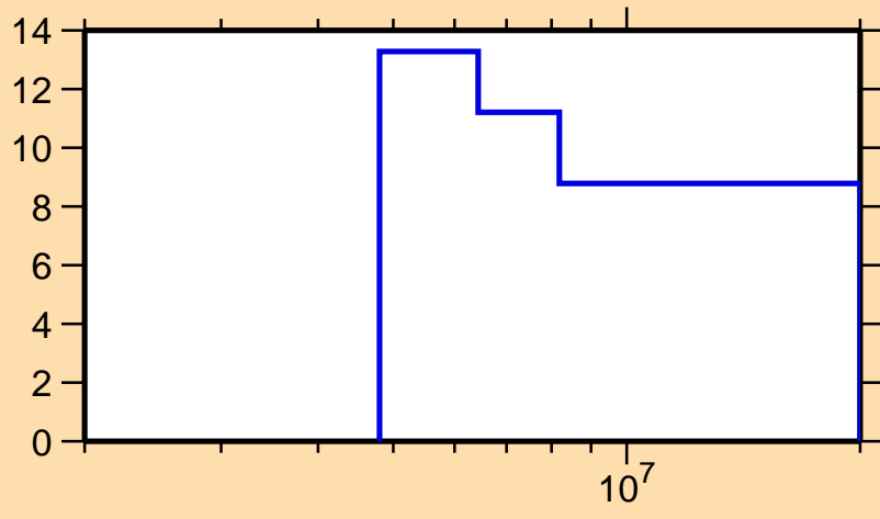
\Delta\sigma/\sigma vs. E for ^{240}\text{Np}(n,\text{nonel.})
