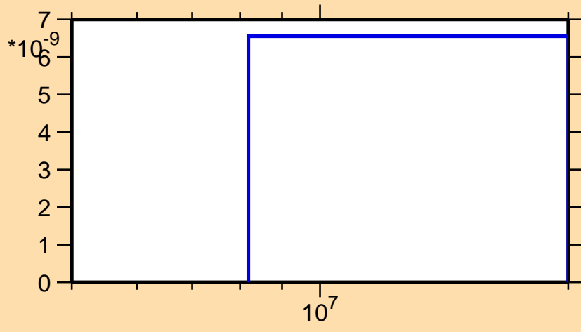
\sigma vs. E for ^{240}\text{Np}(n,2n\alpha)
