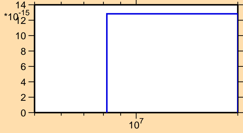
\sigma vs. E for ^{240}\text{Np}(\text{mt } 11)
