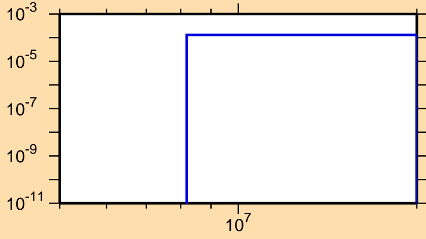
\sigma vs. E for ^{240}\text{Np}(n,d)
