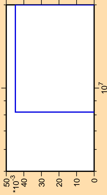
\Delta\sigma/\sigma vs. E for ^{240}\text{Np}(\text{mt } 11)
