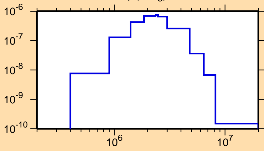
\sigma vs. E for ^{240}\text{Np}(n,n_3)
