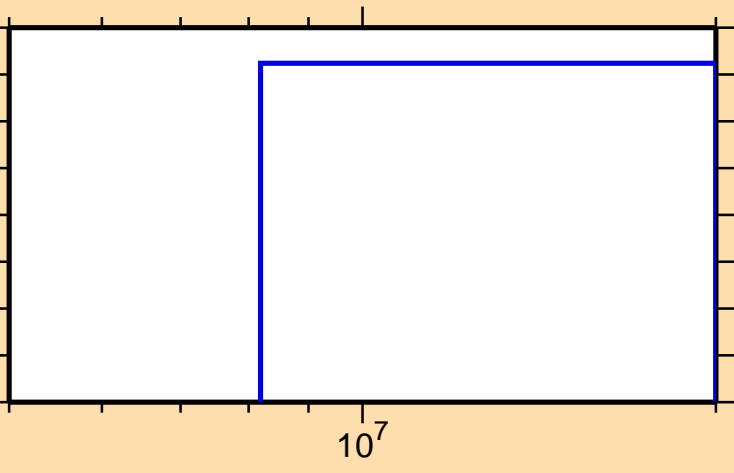
\sigma vs. E for ^{240}\text{Np}(n,3n\alpha)
