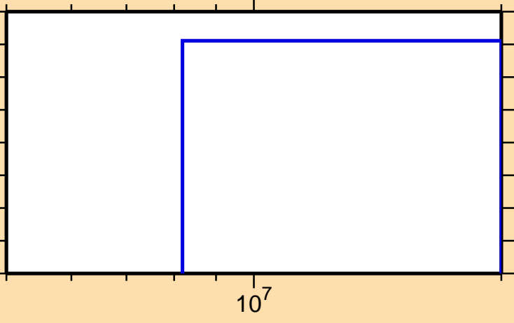
\sigma vs. E for ^{240}\text{Np}(\text{mt } 11)
