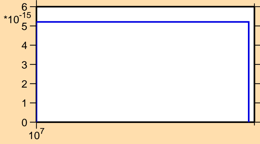
\sigma vs. E for ^{241}\text{Np} (mt 11)
