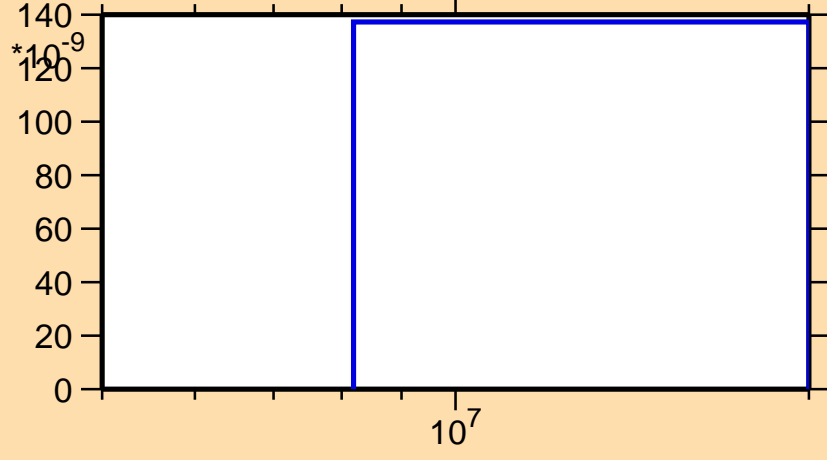
\sigma vs. E for ^{241}\text{Np}(n,nt)
