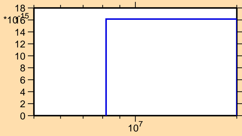
\sigma vs. E for ^{241}\text{Np}(n,3n\alpha)
