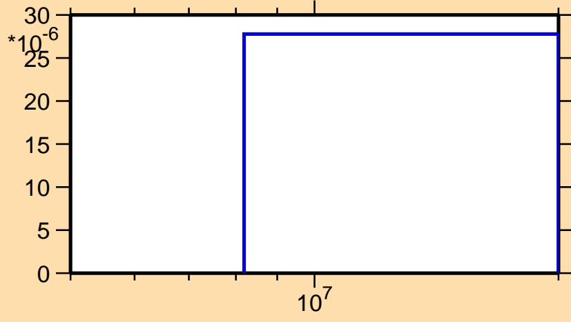
\sigma vs. E for ^{241}\text{Np}(n,t)
