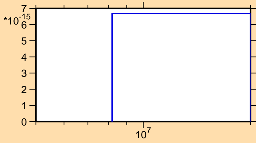
\sigma vs. E for ^{241}\text{Np}(n,\text{He3})
