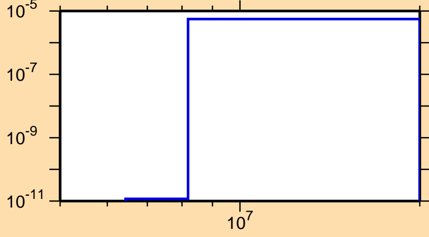
\sigma vs. E for ^{241}\text{Np}(n,n\alpha)
