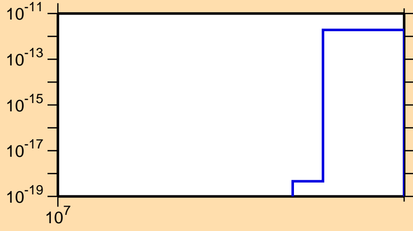
\sigma vs. E for ^{242}\text{Np} (mt 11)
