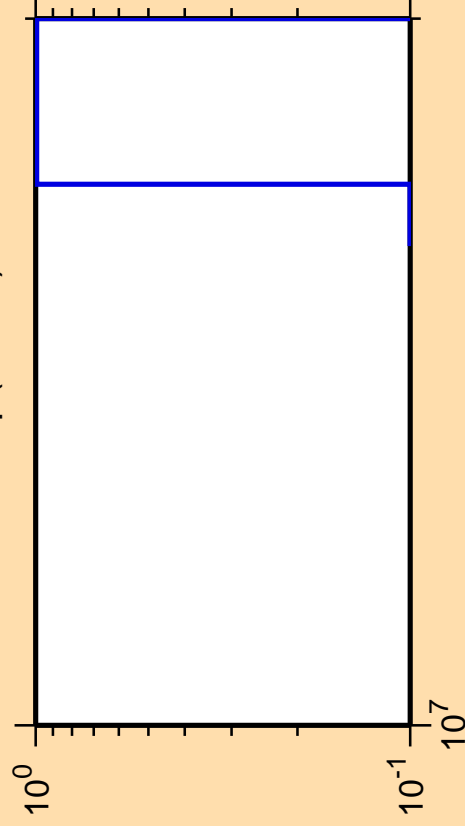
\Delta\sigma/\sigma vs. E for ^{242}\text{Np} (mt 42)
