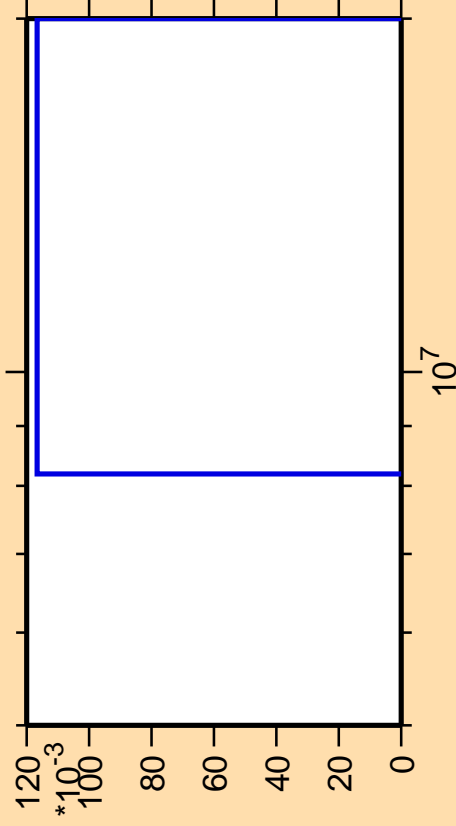
\Delta\sigma/\sigma vs. E for ^{242}\text{Np}(\text{mt } 11)
