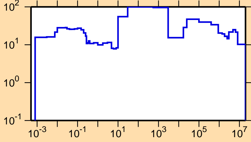
\Delta\sigma/\sigma vs. E for ^{242}\text{Np}(n,tot.)
