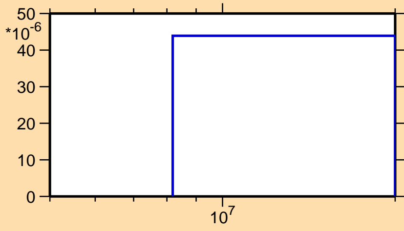
\sigma vs. E for ^{242}\text{Np}(n,np)
