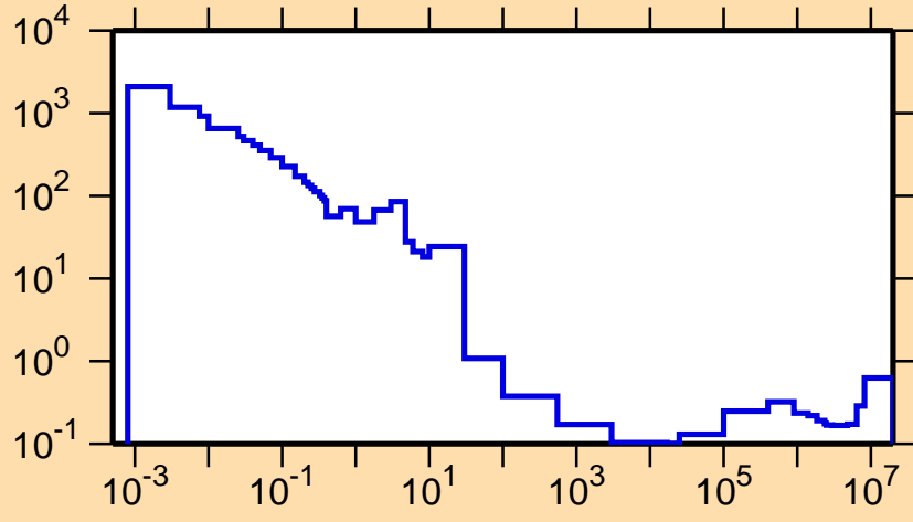
\sigma vs. E for ^{242}\text{Np}(n,f)
