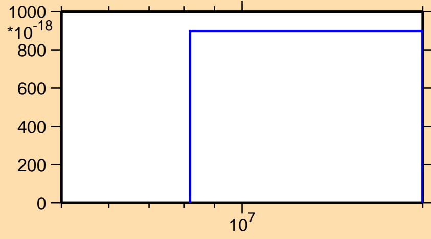
\sigma vs. E for ^{242}\text{Np}(\text{mt } 42)
