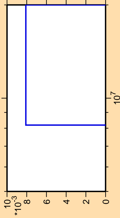
\Delta\sigma/\sigma vs. E for ^{242}\text{Np}(\text{mt } 42)
