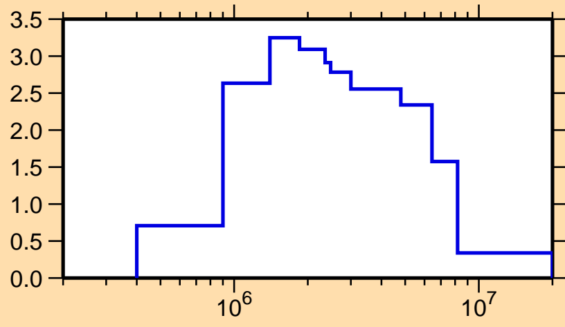
\sigma vs. E for ^{242}\text{Np}(n,n\text{cont.})
