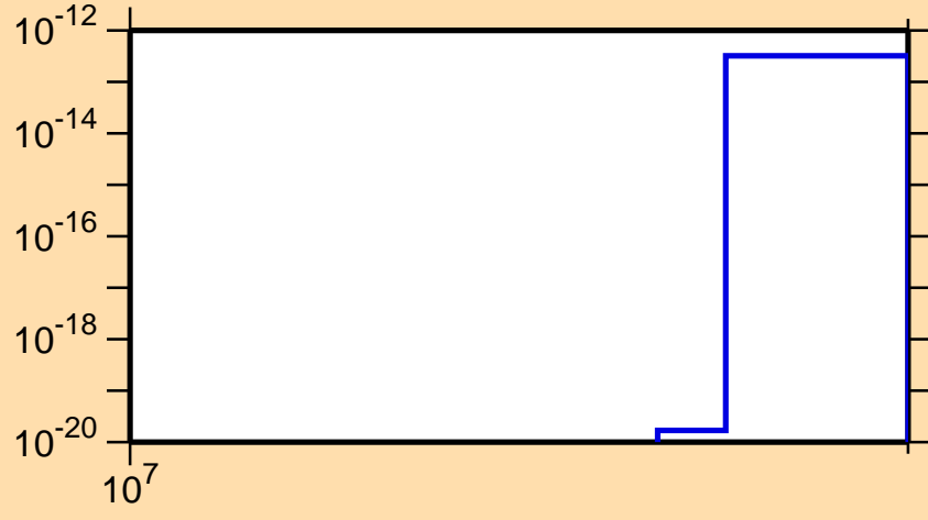
\sigma vs. E for ^{243}\text{Np} (mt 42)
