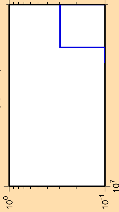
\Delta\sigma/\sigma vs. E for ^{243}\text{Np} (mt 42)
