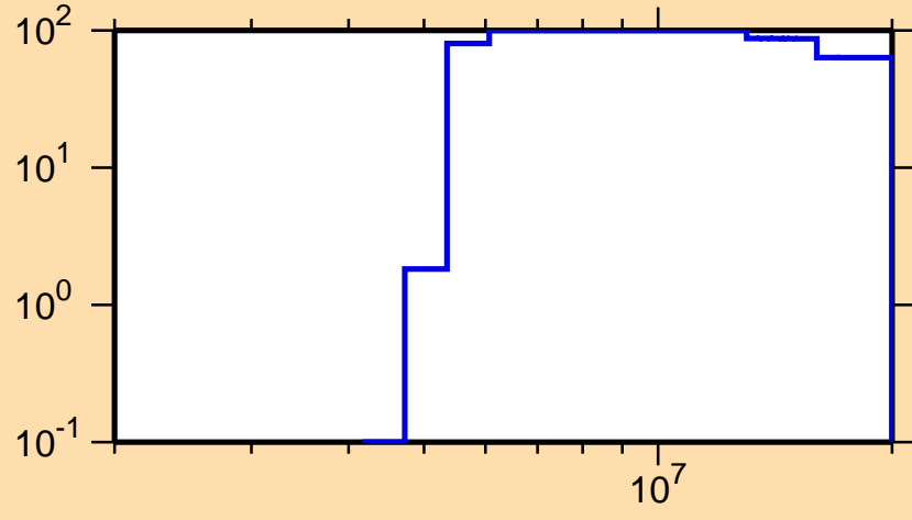
\Delta\sigma/\sigma vs. E for ^{243}\text{Np}(n,p)
