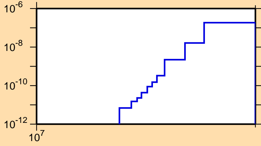
\sigma vs. E for ^{243}\text{Np}(n,2n\alpha)
