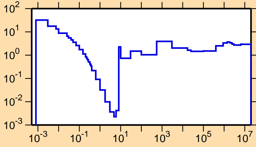
\sigma vs. E for ^{243}\text{Np}(n,\text{nonel.})
