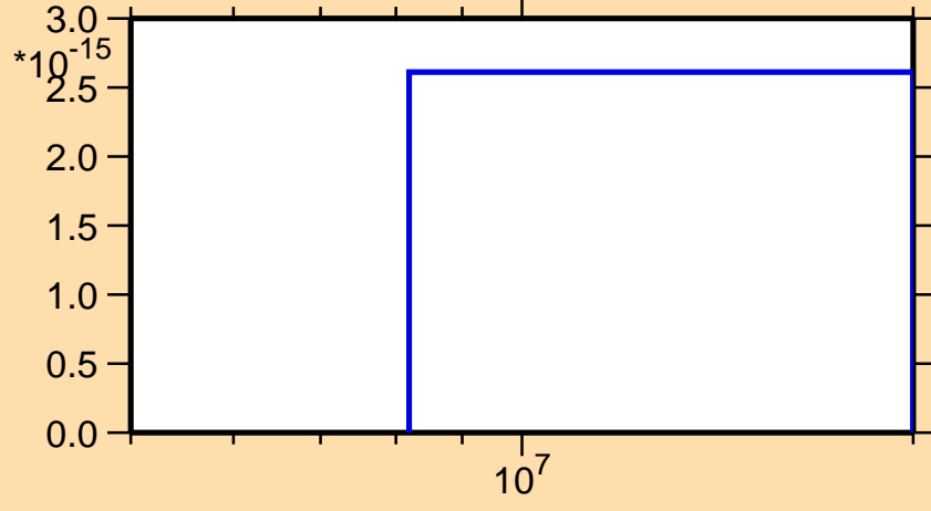
\sigma vs. E for ^{243}\text{Np} (mt 42)
