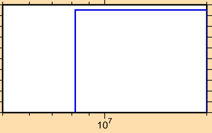
\sigma vs. E for ^{243}\text{Np}(n,\text{nd})
