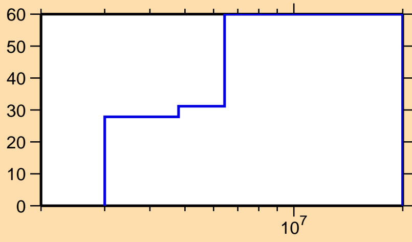
\Delta\sigma/\sigma vs. E for ^{243}\text{Np}(n,\text{inel.})
