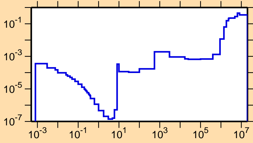
\sigma vs. E for ^{243}\text{Np}(n,f)
