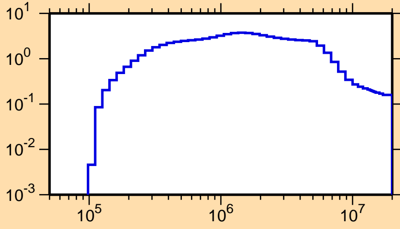
\sigma vs. E for ^{244}\text{Np}(n,n\text{cont.})
