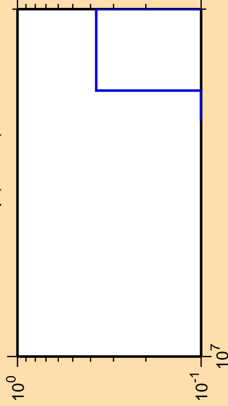
\Delta\sigma/\sigma vs. E for ^{244}\text{Np} (mt 42)
