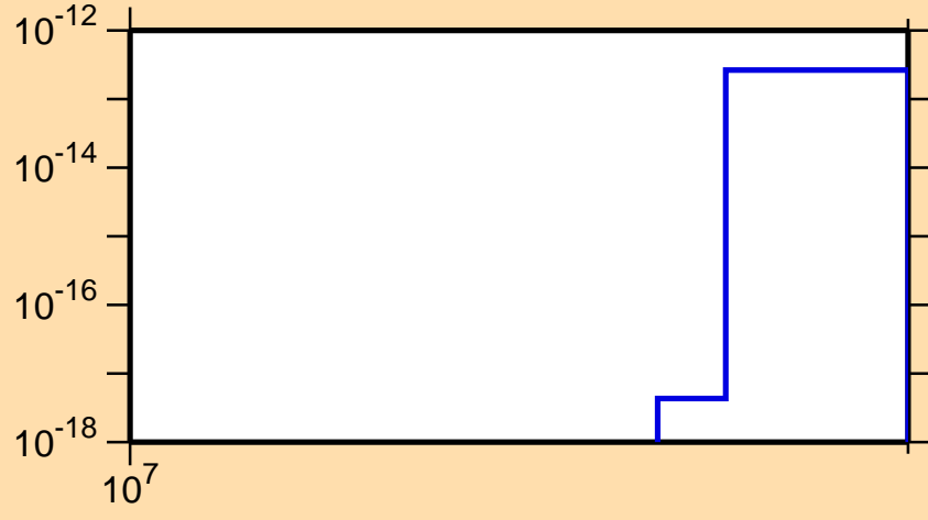
\sigma vs. E for ^{244}\text{Np} (mt 42)
