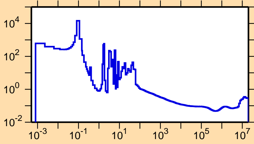
\sigma vs. E for ^{244}\text{Np}(n,f)
