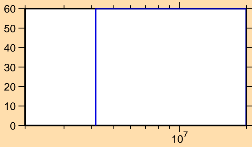
\Delta\sigma/\sigma vs. E for ^{244}\text{Np}(n,\gamma)
