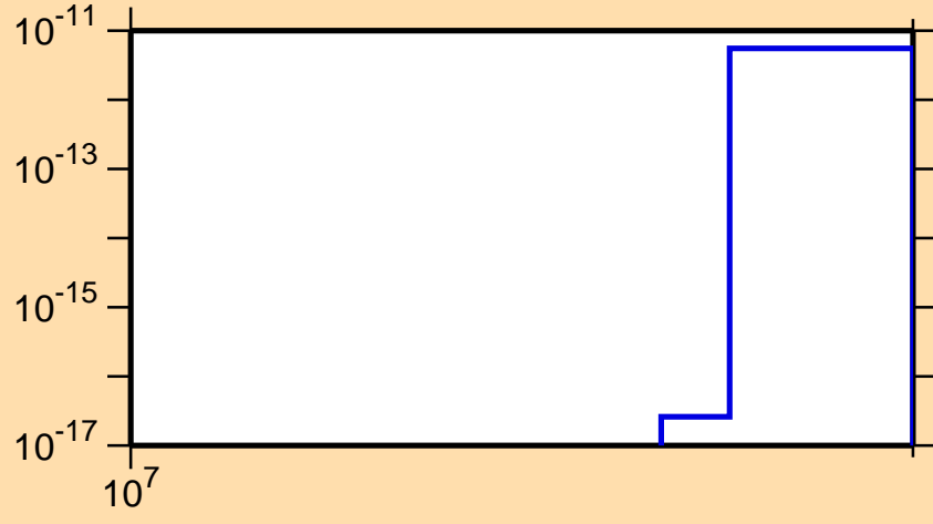
\sigma vs. E for ^{244}\text{Np}(\text{mt } 11)
