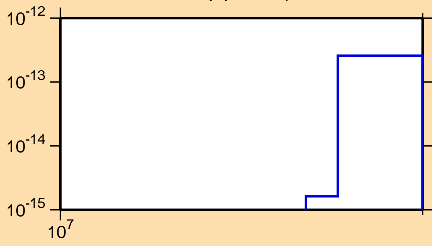
\sigma vs. E for ^{244}\text{Np}(n,\text{He3})
