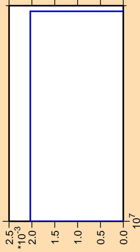
\Delta\sigma/\sigma vs. E for ^{244}\text{Np} (mt 42)
