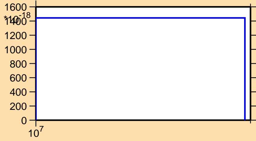
\sigma vs. E for ^{244}\text{Np} (mt 42)
