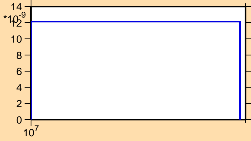
\sigma vs. E for ^{244}\text{Np}(n,2np)
