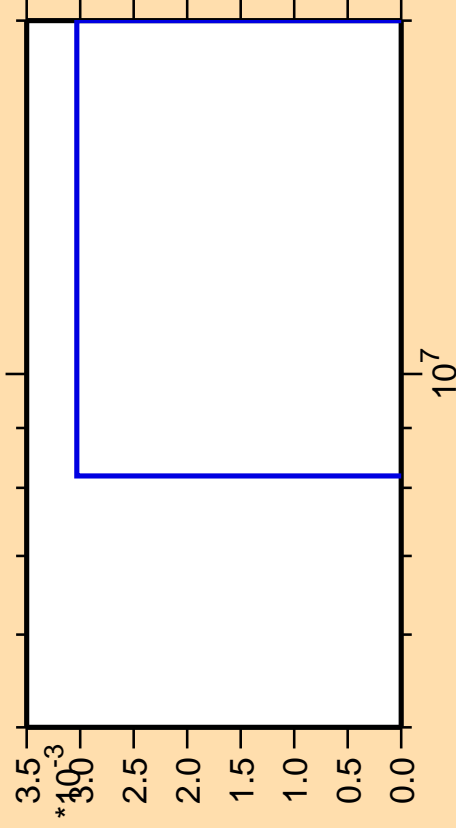
\Delta\sigma/\sigma vs. E for ^{244}\text{Np}(\text{mt } 42)
