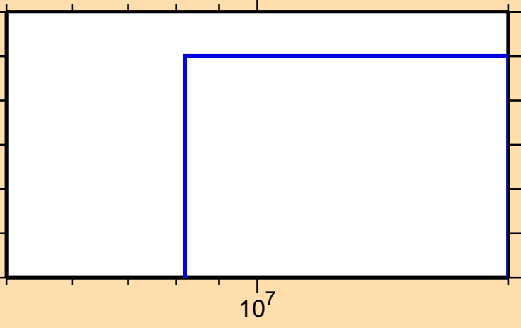
\sigma vs. E for ^{244}\text{Np}(n,np)
