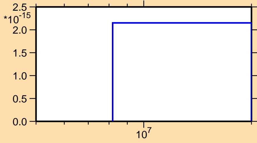
\sigma vs. E for ^{244}\text{Np}(\text{mt } 42)
