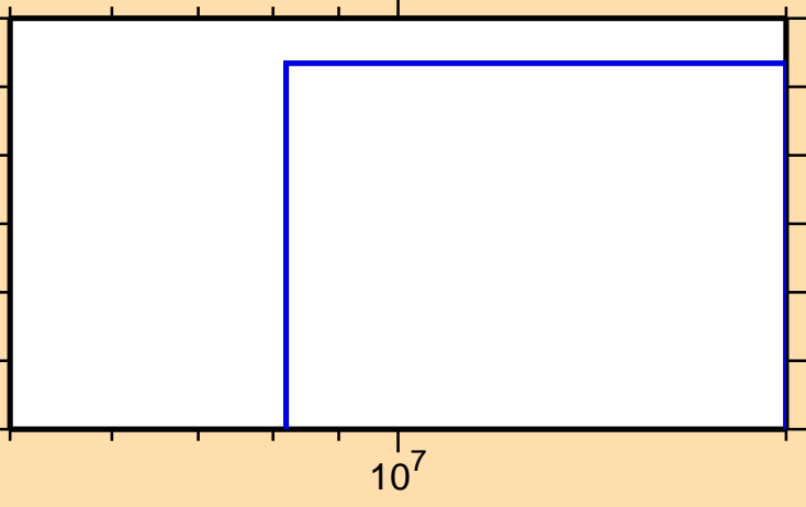
\sigma vs. E for ^{244}\text{Np}(n,2np)
