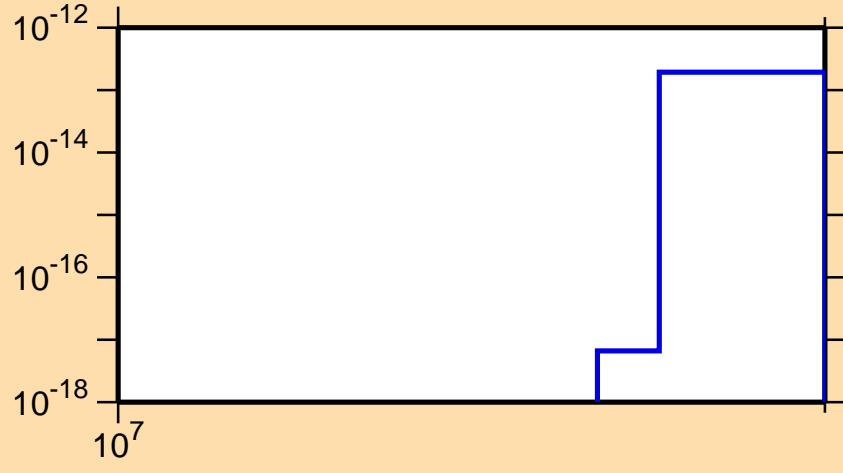
\sigma vs. E for ^{245}\text{Np} (mt 42)
