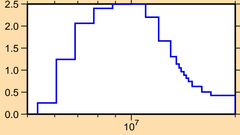
\sigma vs. E for ^{245}\text{Np}(n,2n)
