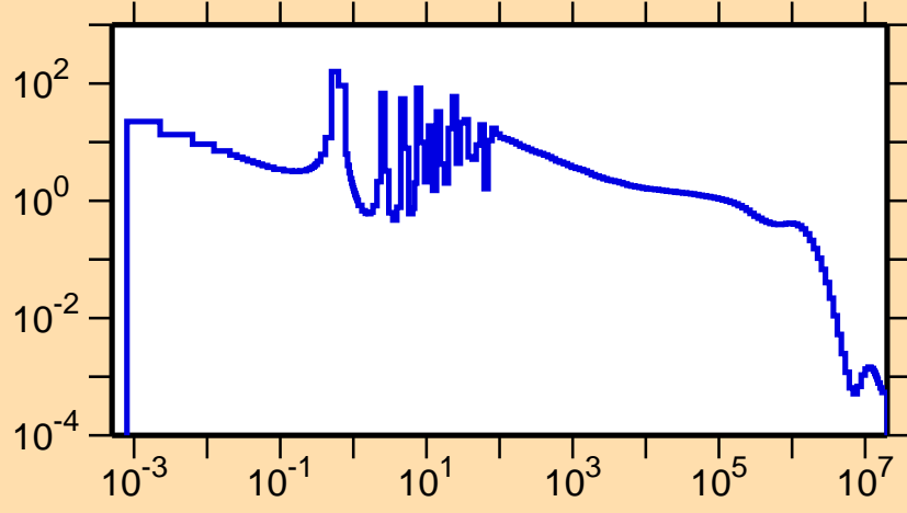
\sigma vs. E for ^{245}\text{Np}(n,\gamma)
