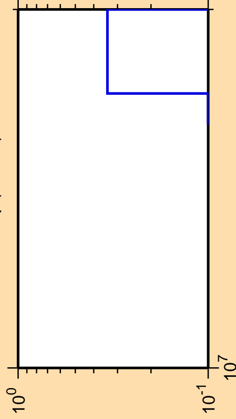
\Delta\sigma/\sigma vs. E for ^{245}\text{Np} (mt 42)
