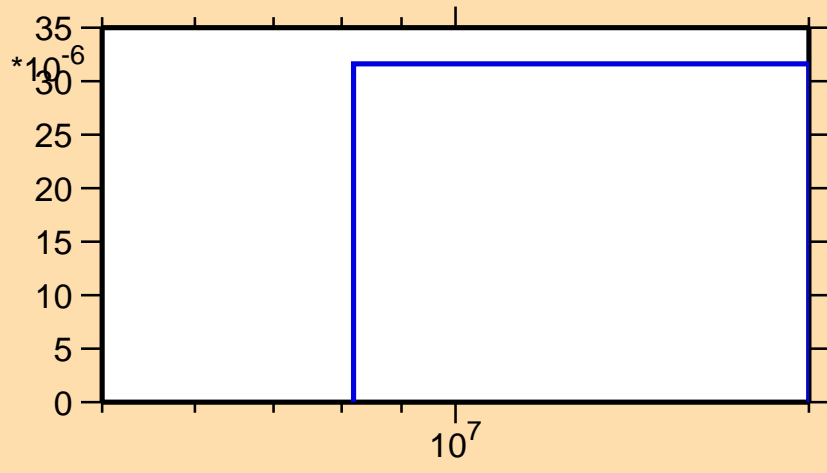
\sigma vs. E for ^{245}\text{Np}(n,d)
