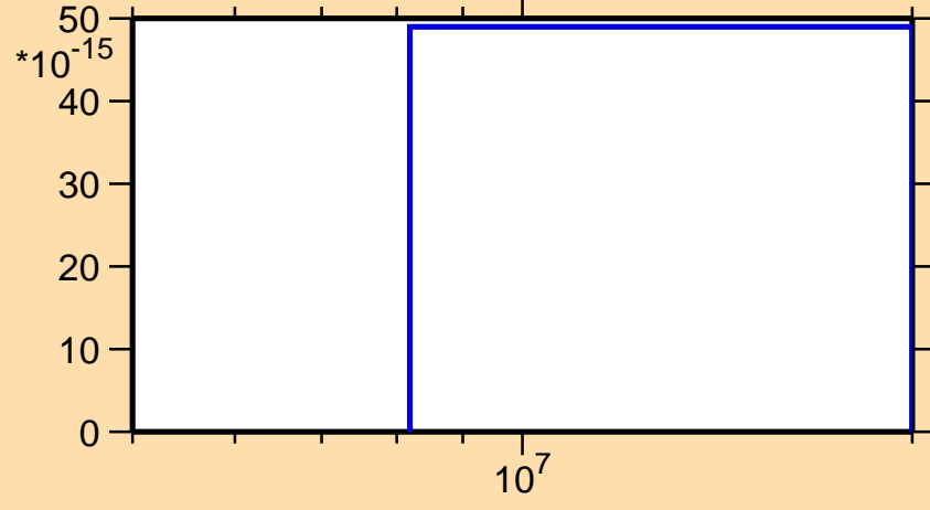
\sigma vs. E for ^{245}\text{Np}(\text{mt } 11)
