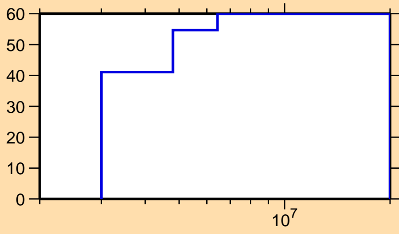
\Delta\sigma/\sigma vs. E for ^{245}\text{Np}(n,n\text{cont.})
