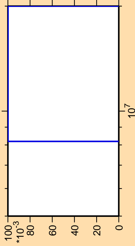
\Delta\sigma/\sigma vs. E for ^{245}\text{Np}(\text{mt } 11)
