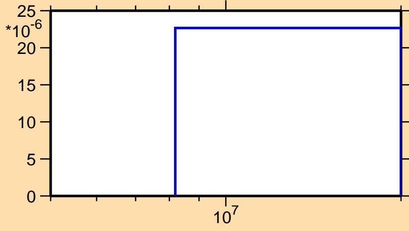
\sigma vs. E for ^{245}\text{Np}(n,t)
