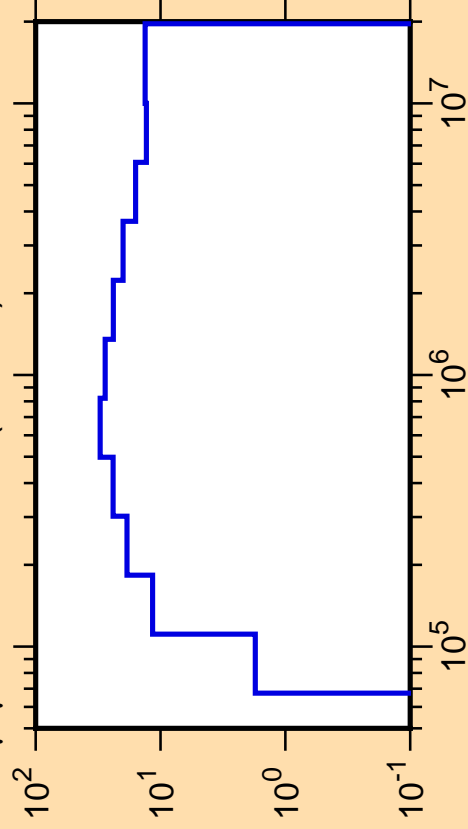
\Delta\mu/\mu vs. E for ^{15}\text{O}(\text{mt251})
