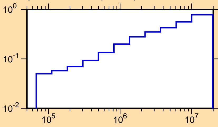
\mu vs. E for ^{15}\text{O}(\text{mt251})
