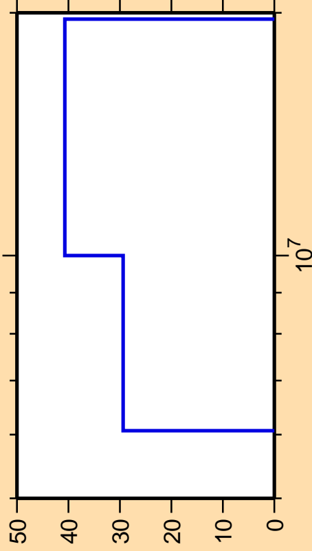
\Delta\sigma/\sigma vs. E for ^{15}\text{O}(n,n_4)
