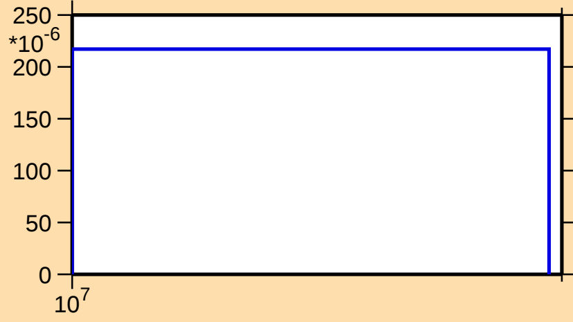
\sigma vs. E for ^{18}\text{O}(\text{n,d})
