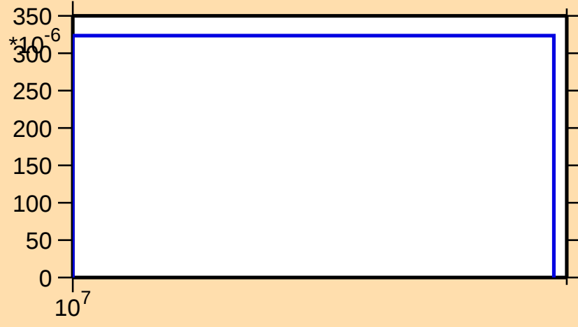
\sigma vs. E for ^{18}\text{O}(\text{n,p})
