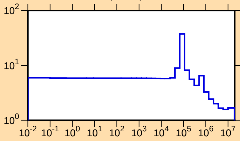
\sigma vs. E for ^{18}\text{O}(\text{n,tot.})
