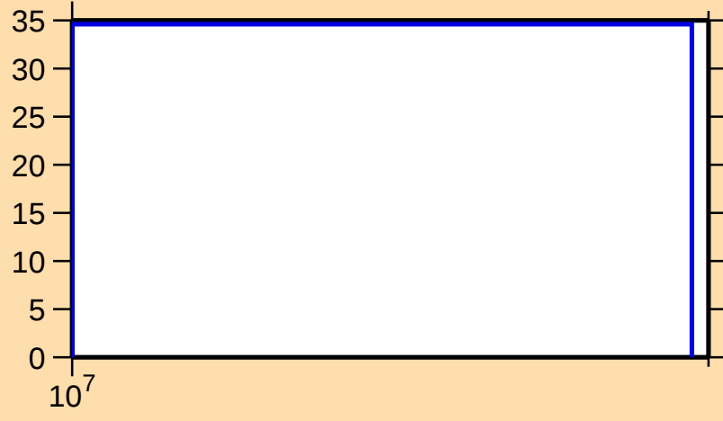
\Delta\sigma/\sigma vs. E for ^{18}\text{O}(n,p)
