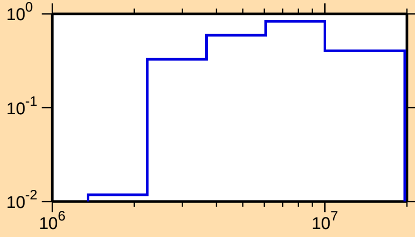
\sigma vs. E for ^{18}\text{O}(\text{n,inel.})
