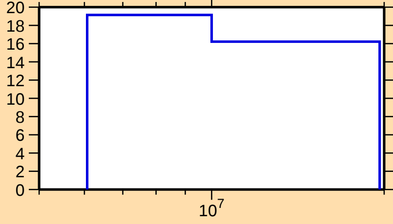
\Delta\sigma/\sigma vs. E for ^{18}\text{O}(\text{n},2\text{n})
