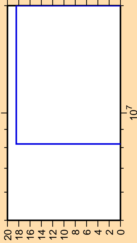
\Delta\sigma/\sigma vs. E for ^{20}\text{O}(n,3n)
