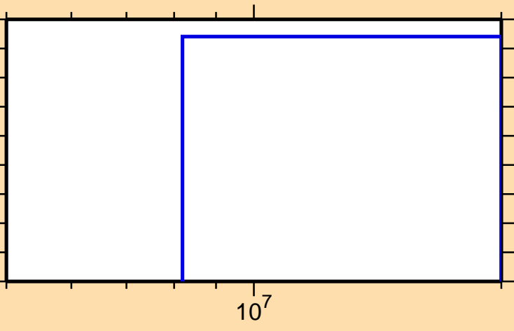
\sigma vs. E for ^{20}\text{O}(n,n\text{cont.})
