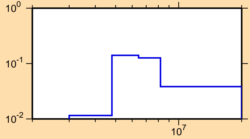
\sigma vs. E for ^{20}\text{O}(n,n_3)
