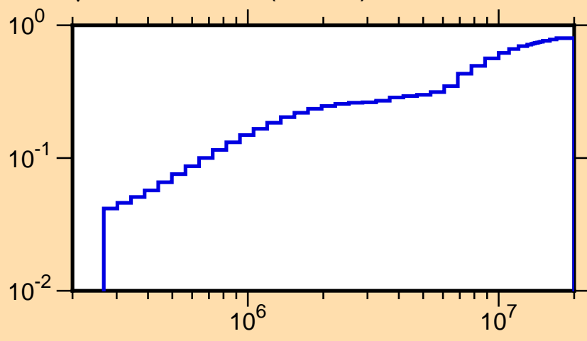
\mu vs. E for ^{22}\text{O}(\text{mt251})
